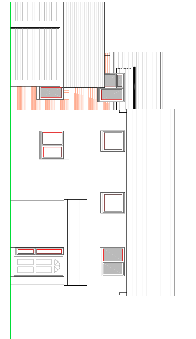
FRONT ELEVATION
