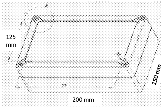
Dimensions and illustration of IP enclosure
