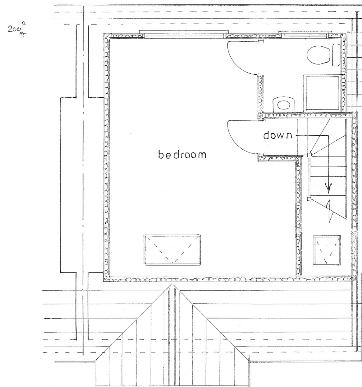
2nd floor plan 1 : 50
