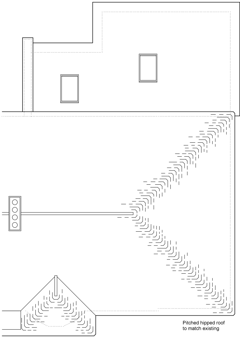
Roof Plan
