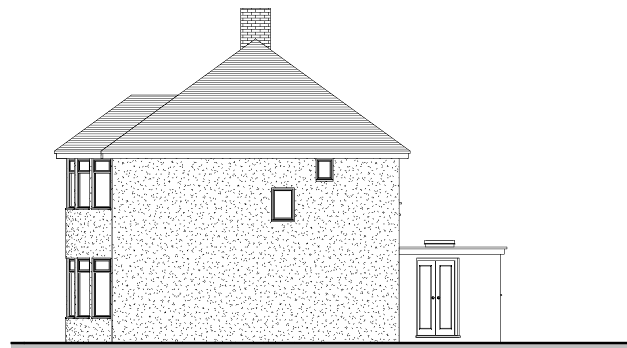
3 North (Side) Elevation Existing 1 : 100
