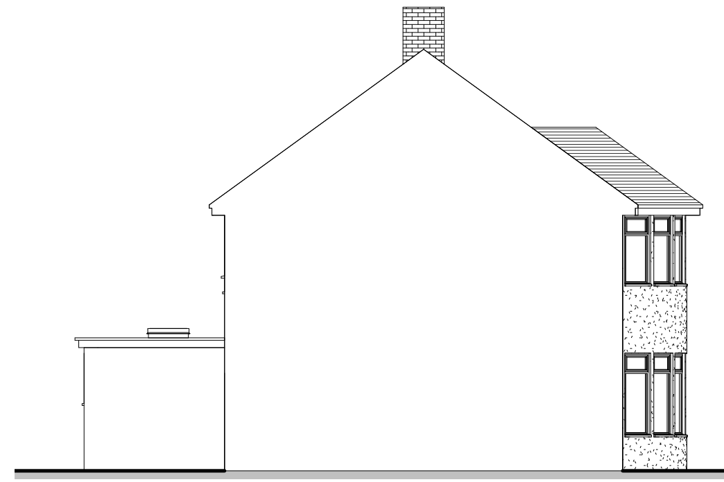
1 South (Side) Elevation Existing 1 : 100
