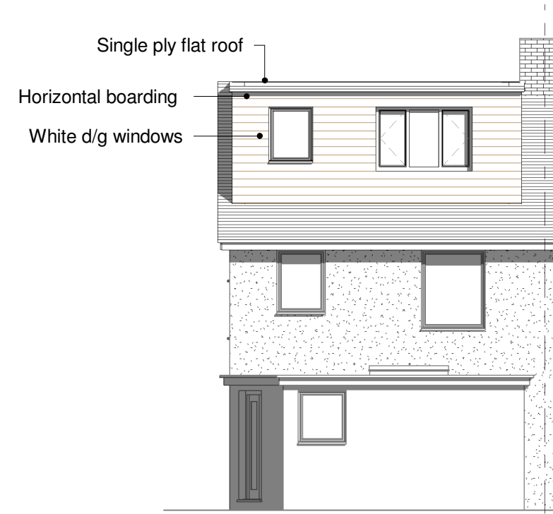
8 West (Rear) Elevation Proposed 1 : 100
