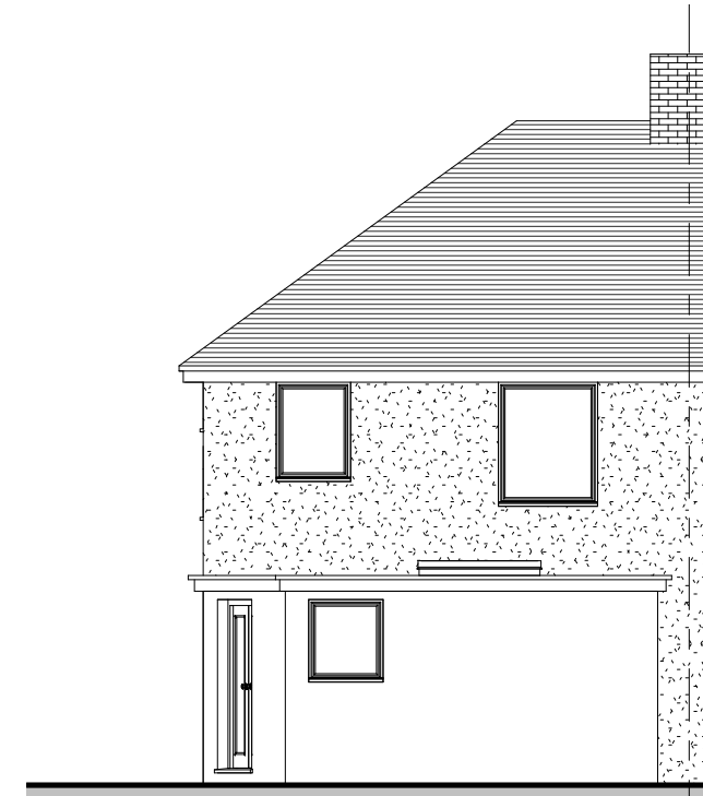
6 East Front Elevation Proposed 1 : 100
