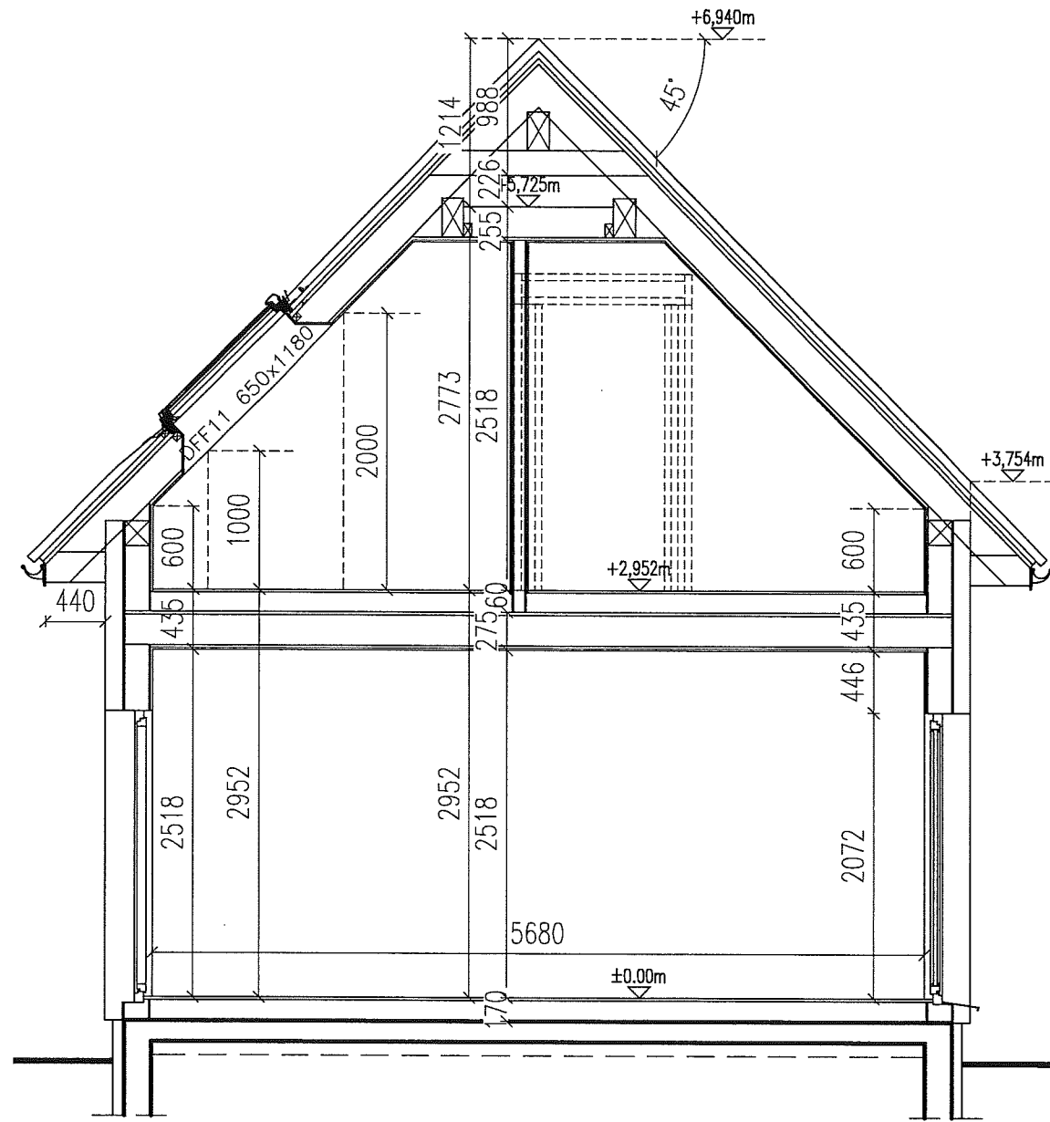
SECTION B-B
