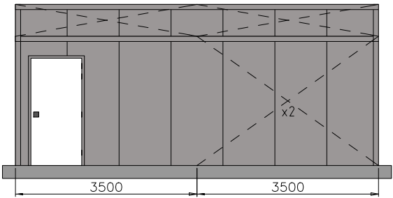
Left Elevation (Internal)
