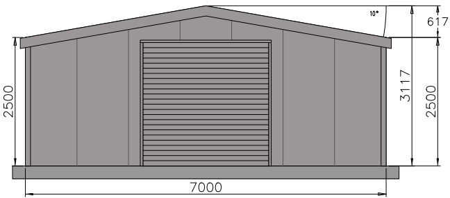
Front Elevation (External)
