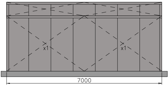
Right Elevation (External)
