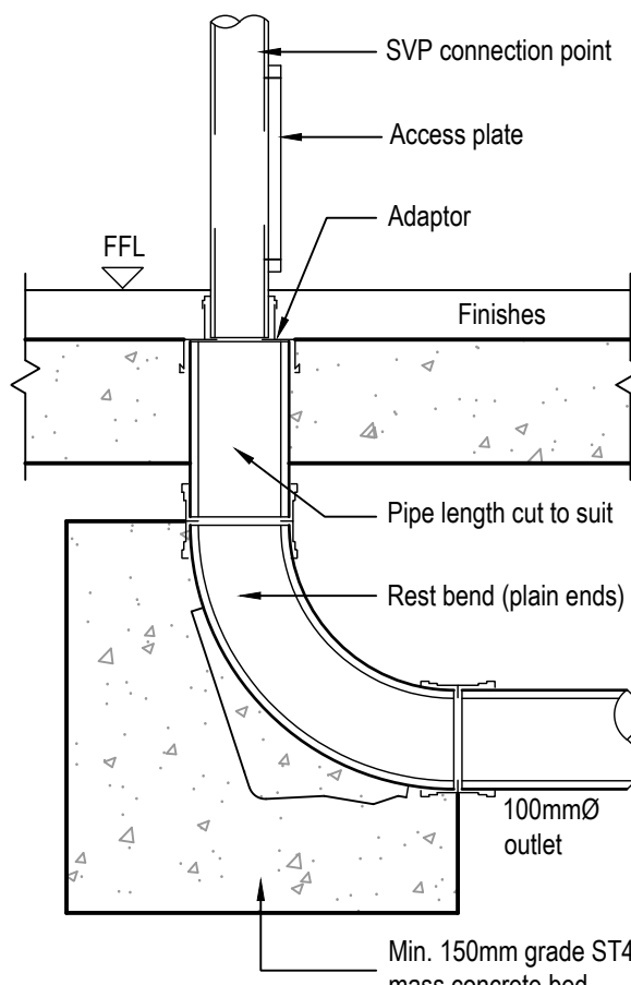
Roddable Internal SVP Detail SCALE = 1:10
