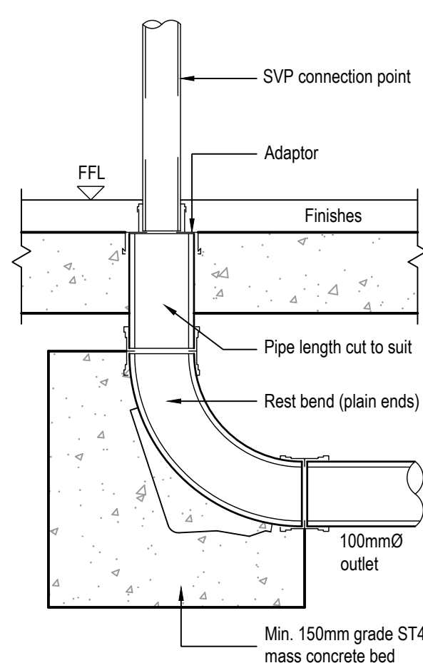
Non-Roddable Internal SVP Detail SCALE = 1:10
