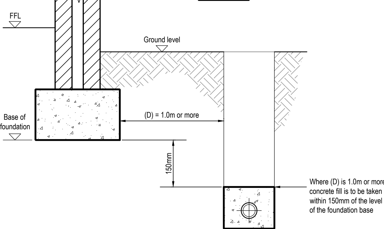
Protection of Pipes Adjacent to Building Detail SCALE = 1:20
