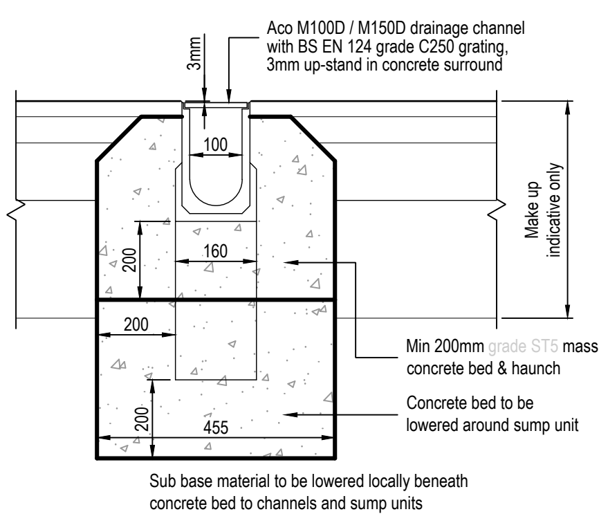
Aco M100D / M150D Drainage Channel Construction Detail
