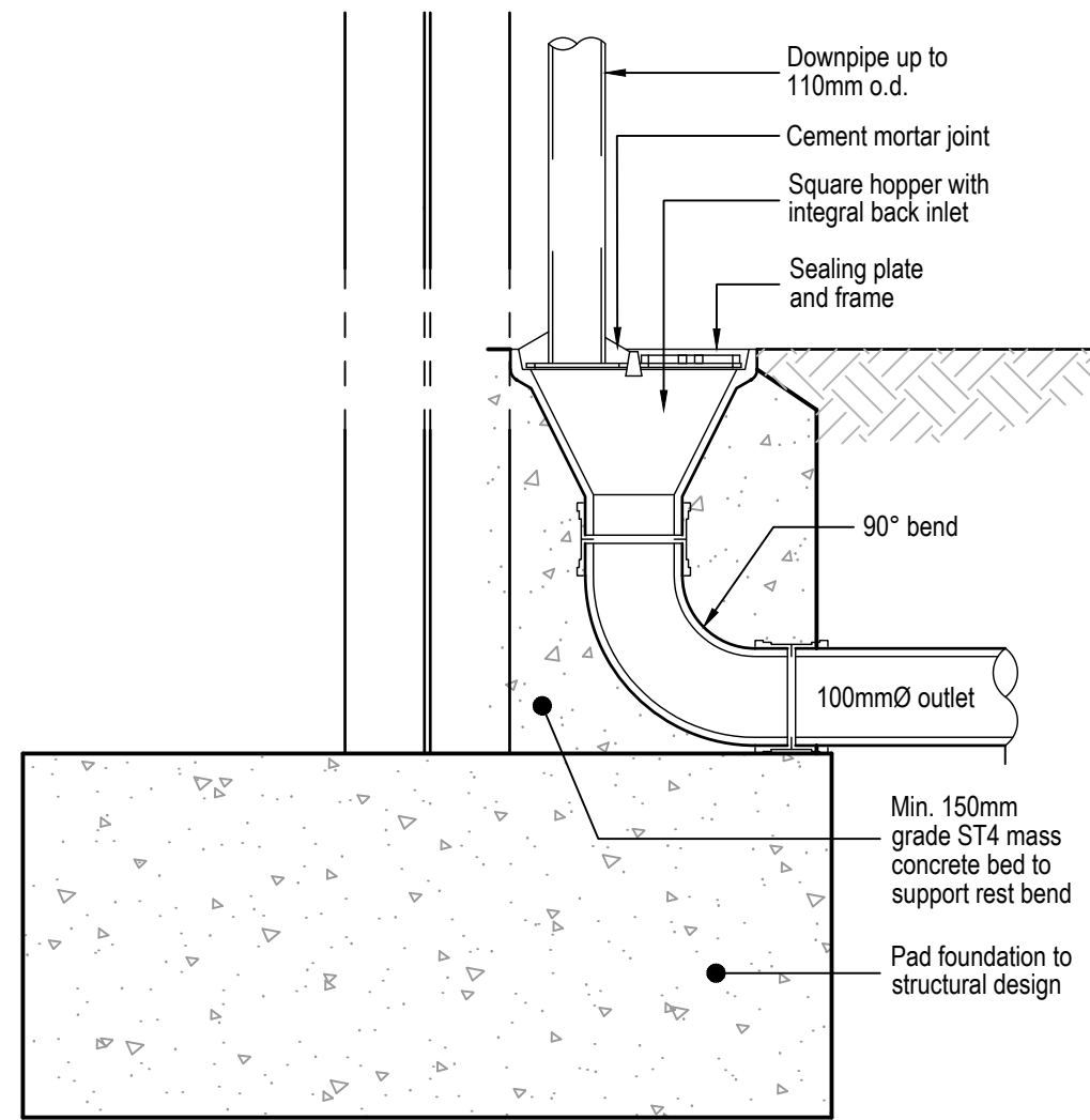
Roddable RWP Connection Detail SCALE = 1:10
