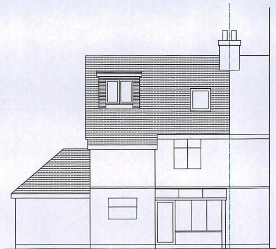
Proposed Rear Elevation (South))
