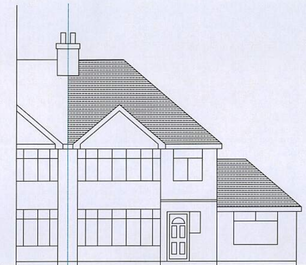
Existing Front Elevation (North)
