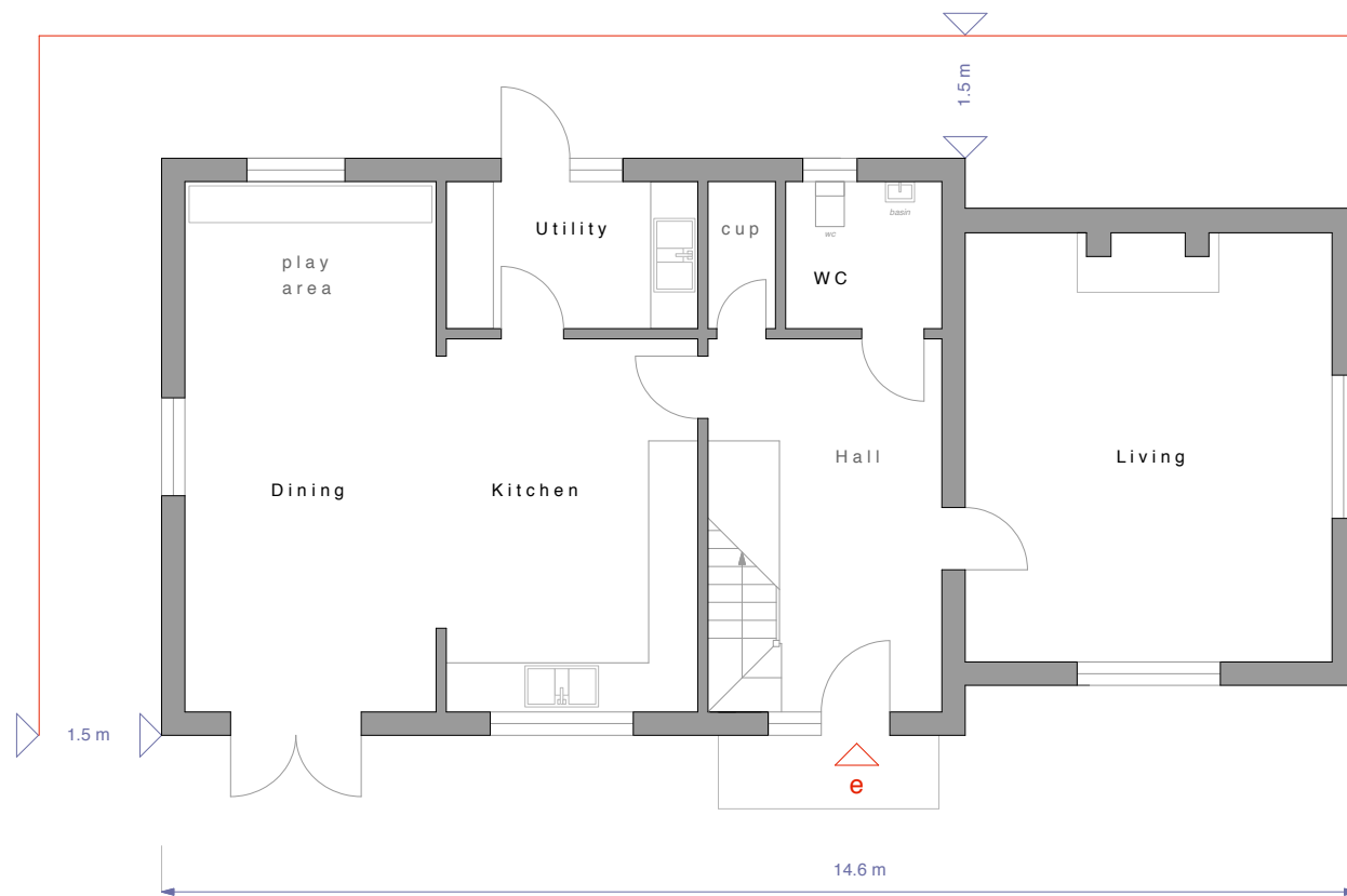
Proposed GF Plan at 1:100 scale
