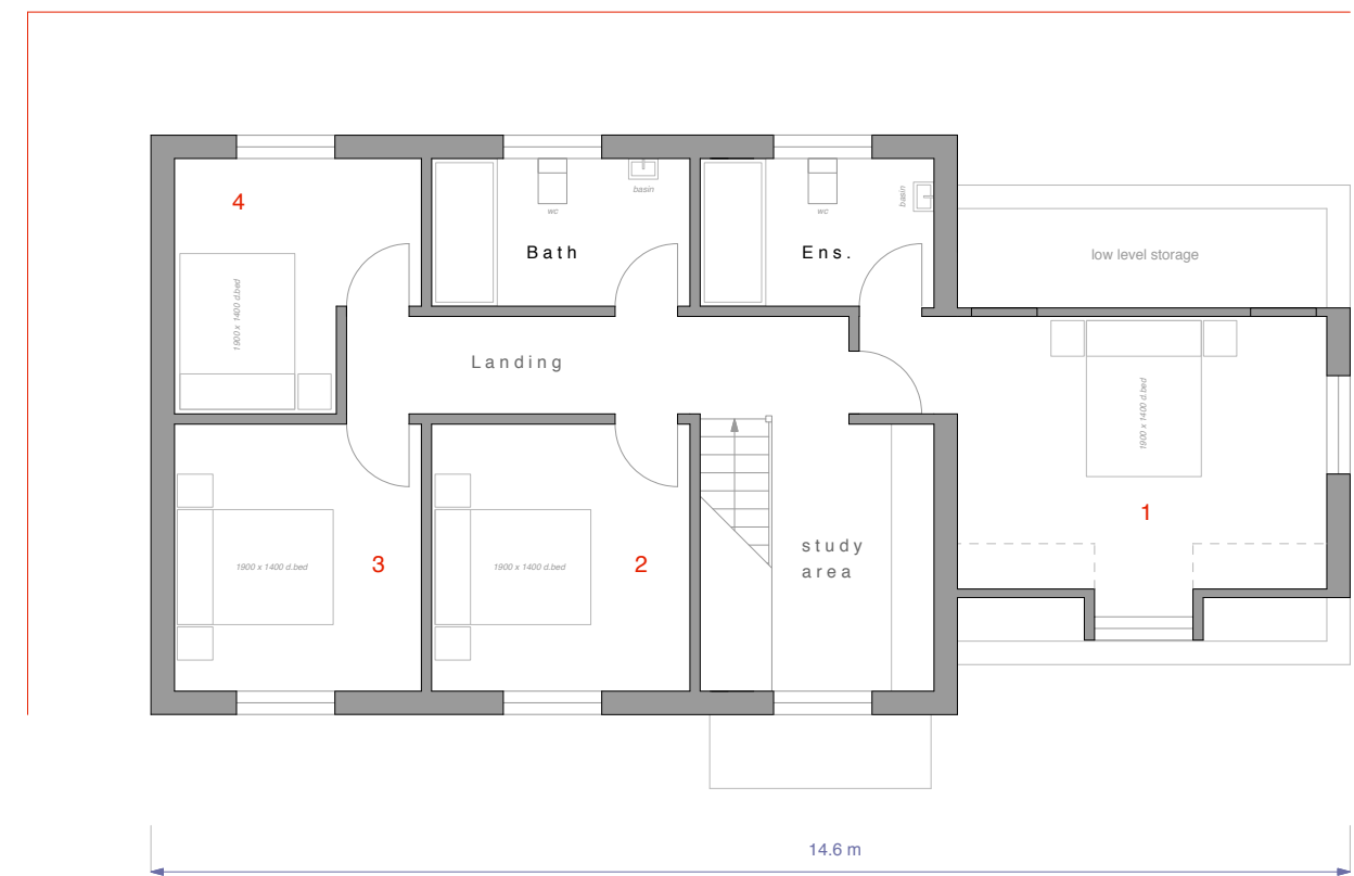
Proposed FF Plan at 1:100 scale
