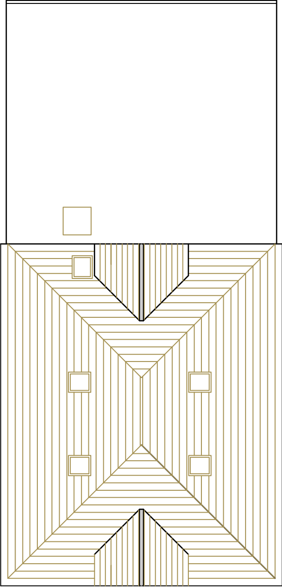
PROPOSED NEW ROOF PLAN 1:100
