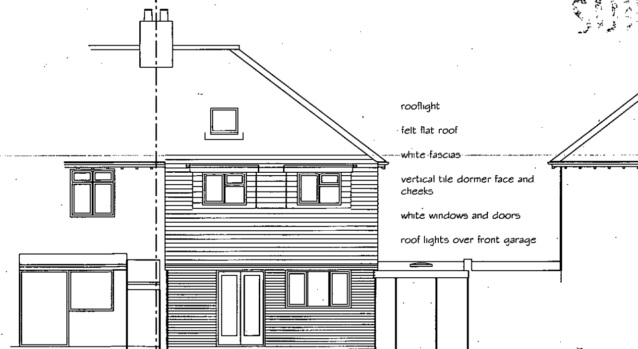
East Elevation
