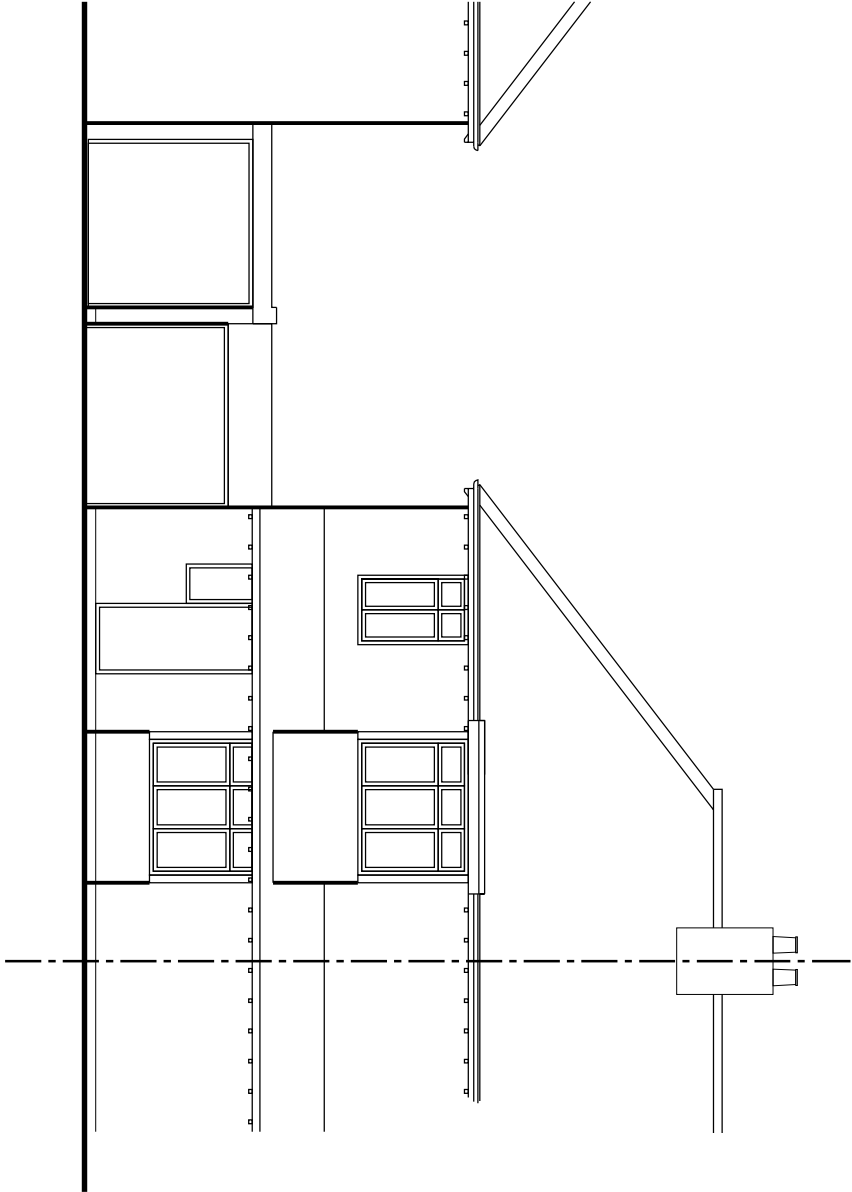
South Elevation
