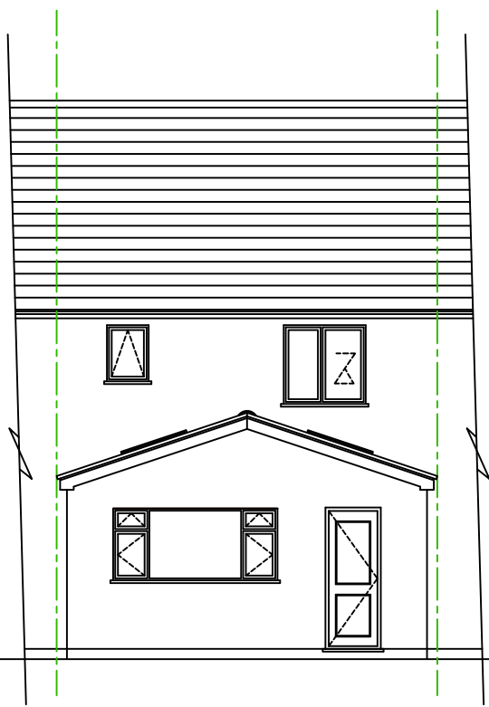
Proposed NNE Elevation
