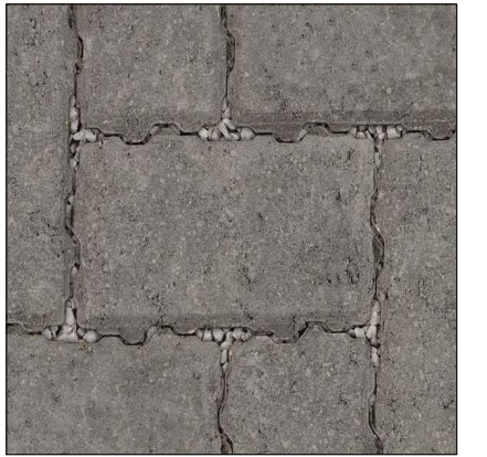
12 Concrete paving to road/visitor parking Product: Marshall Priora Permeable - Staggered bond Colour/ Finish: Charcoal Size: 200 x 100 x 80mm
