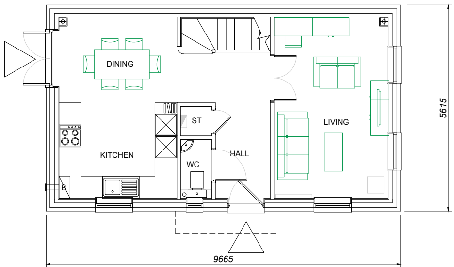
Plot 92 310 GROUND FLOOR PLAN
