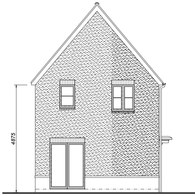
SIDE ELEVATION
