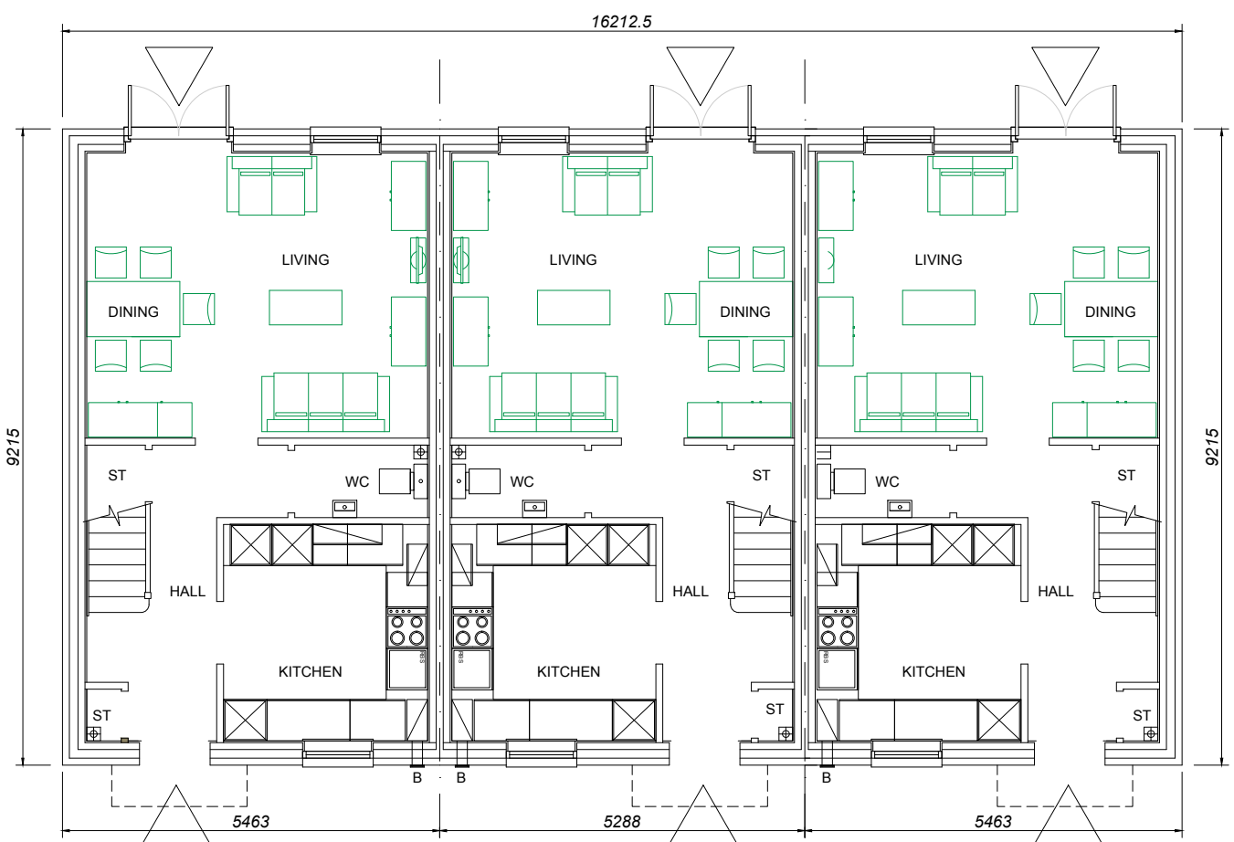
Plot 75 A3 Plot 76 A3 Plot 82 A3 GROUND FLOOR PLAN
