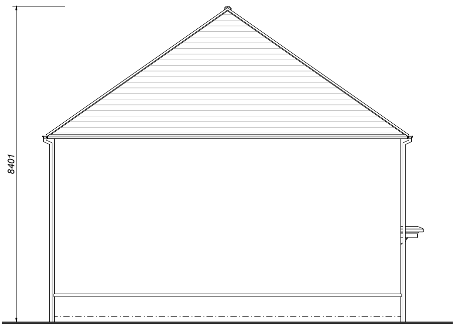
Plot 75 A3 SIDE ELEVATION
