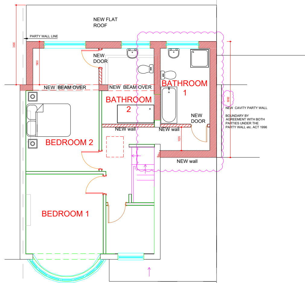
FIRST FLOOR - PROPOSED
