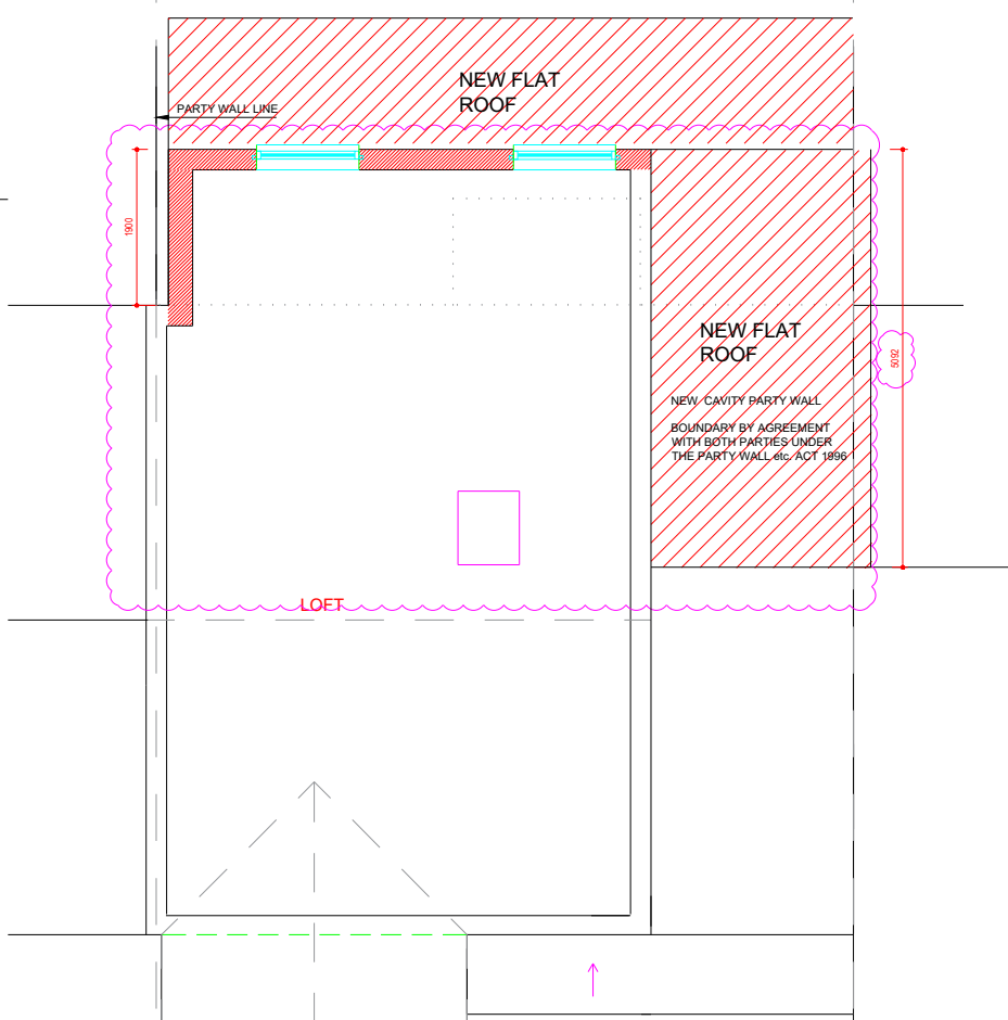
LOFT - PROPOSED
