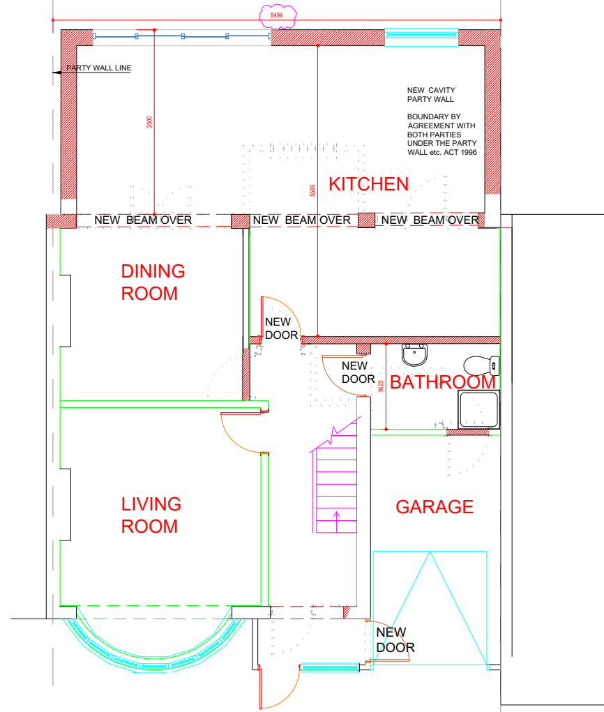
GROUND FLOOR - PROPOSED
