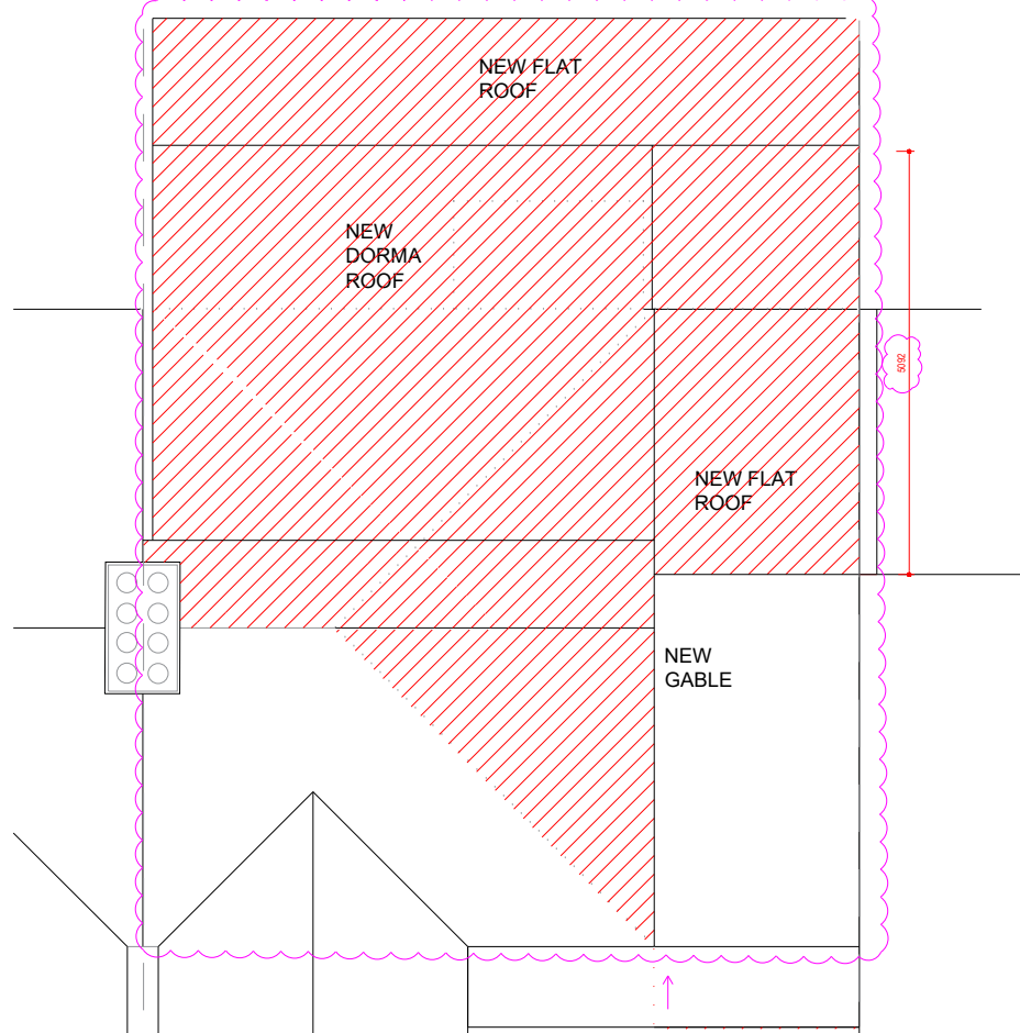
ROOF PLAN - PROPOSED
