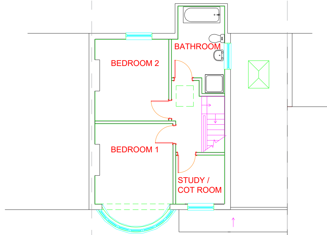
FIRST FLOOR - EXISTING
