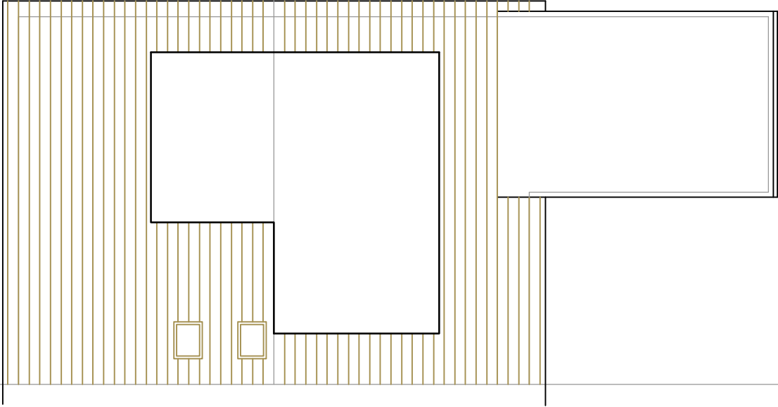
PROPOSED ROOF PLAN 1:100
