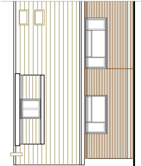
PROPOSED NORTH ELEVATION 1:100
