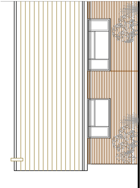
EXISTING NORTH ELEVATION 1:100
