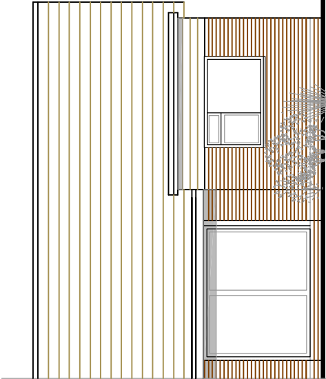
EXISTING SOUTH ELEVATION 1:100
