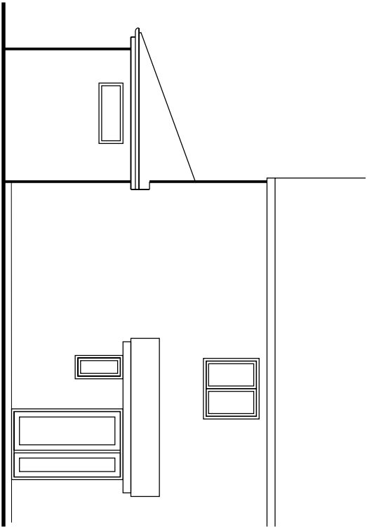
Part South West Elevation
