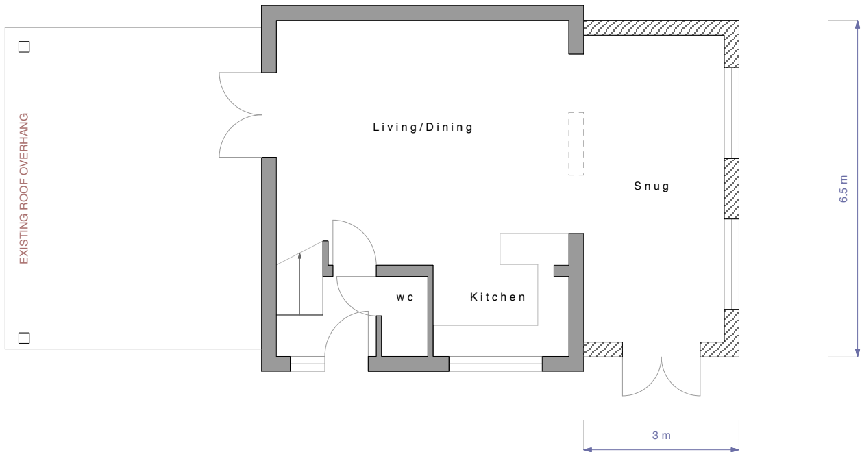
Proposed GF Plan at 1:100 scale
