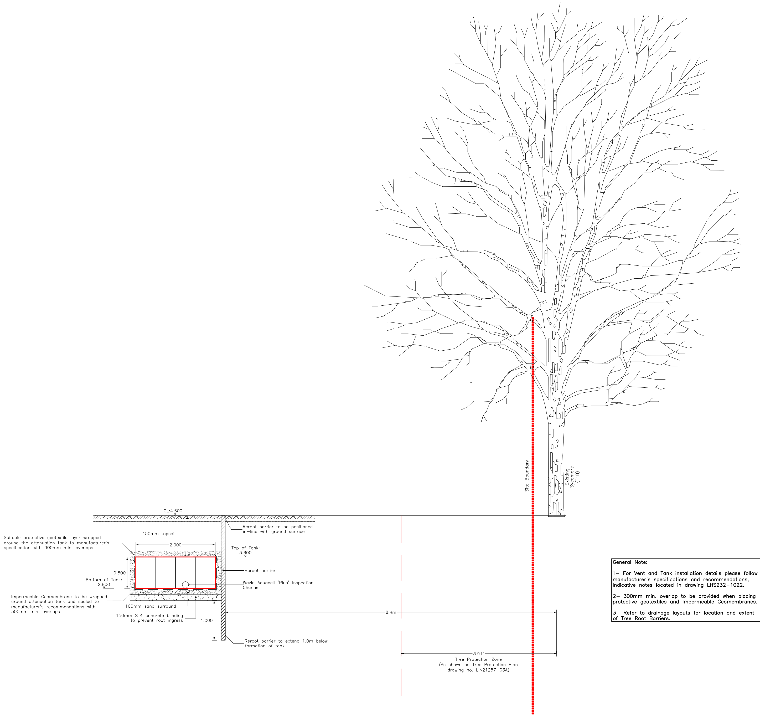
Reroot Barrier Detail Scale 1:50
