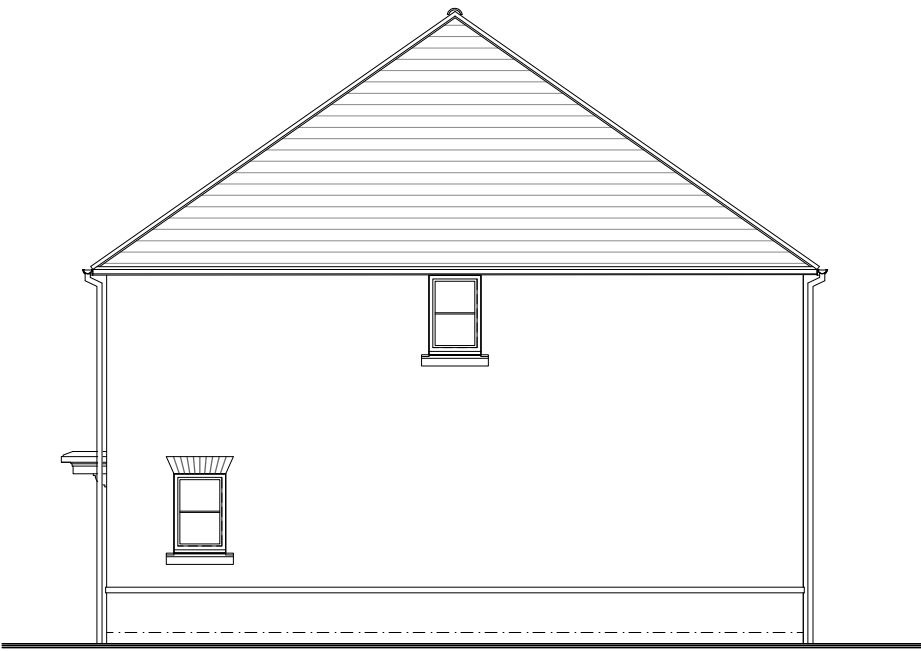
Plot 99 303 SIDE ELEVATION
