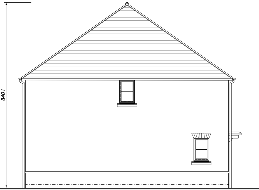
Plot 49 303 SIDE ELEVATION
