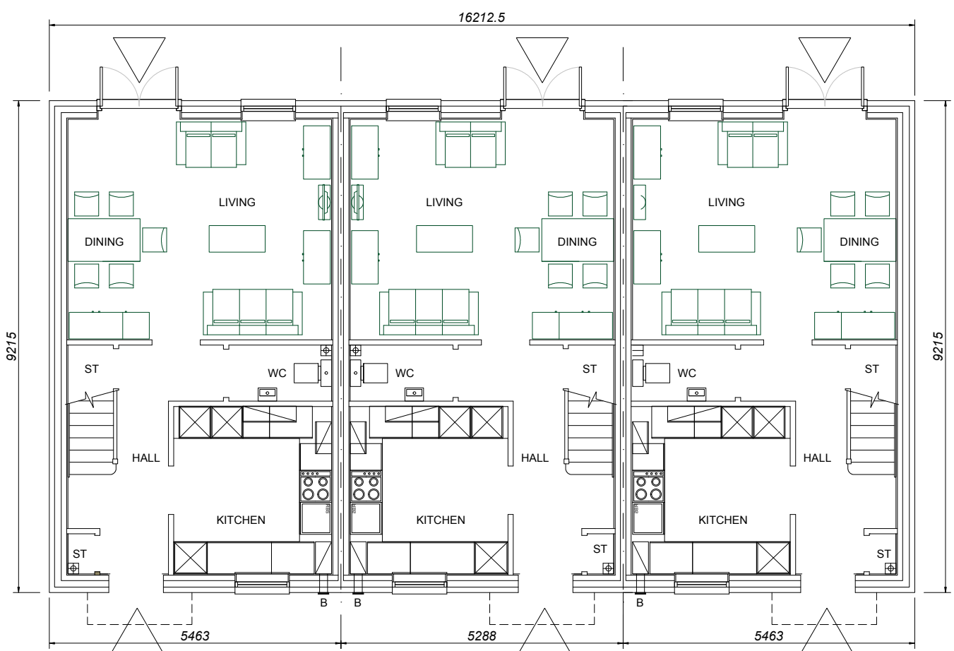
Plot 71 A3 Plot 72 A3 Plot 73 A3 GROUND FLOOR PLAN
