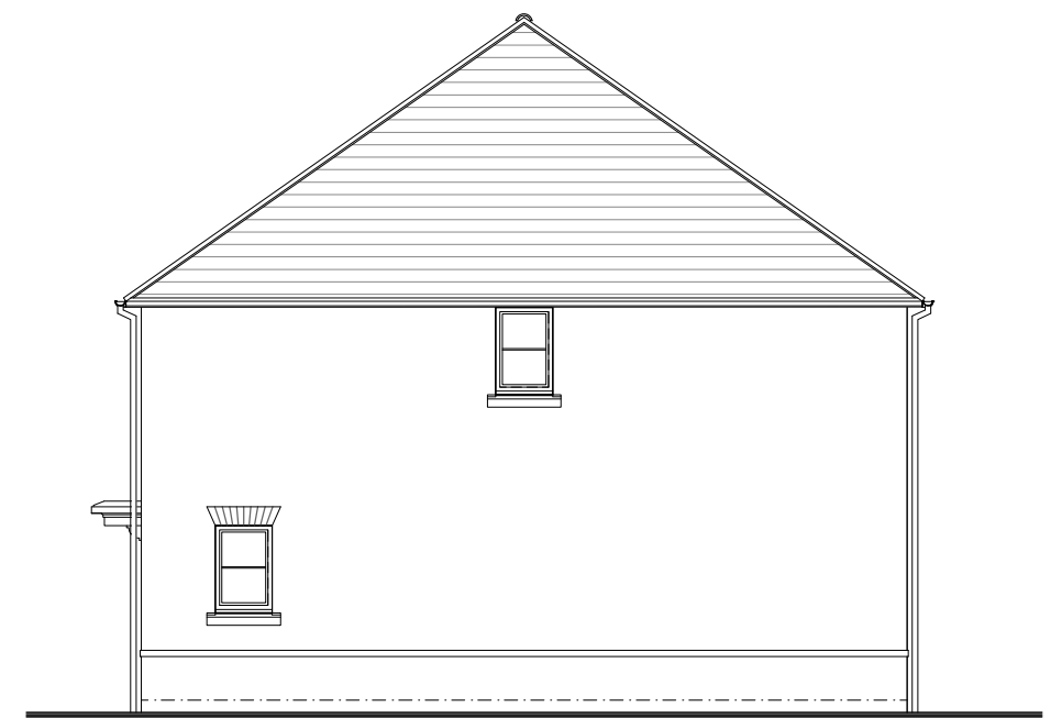
Plot 12 303 SIDE ELEVATION
