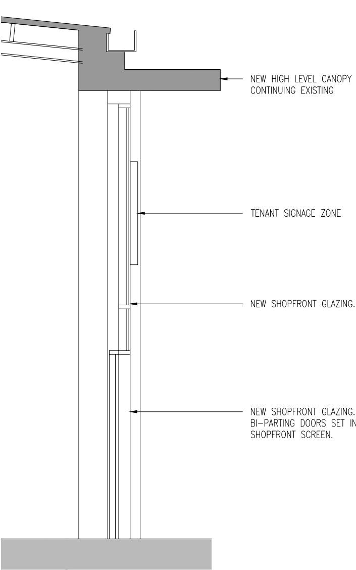
SECTION B-B (PETS AT HOME)
