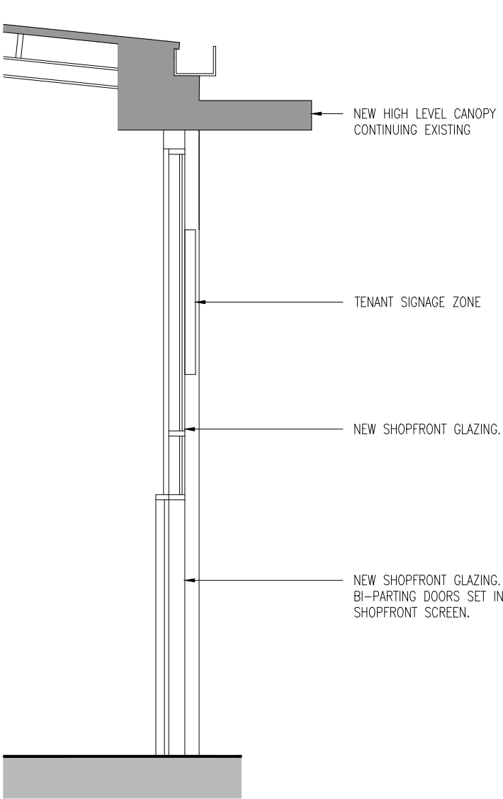
SECTION A-A (CARPETRIGHT)
