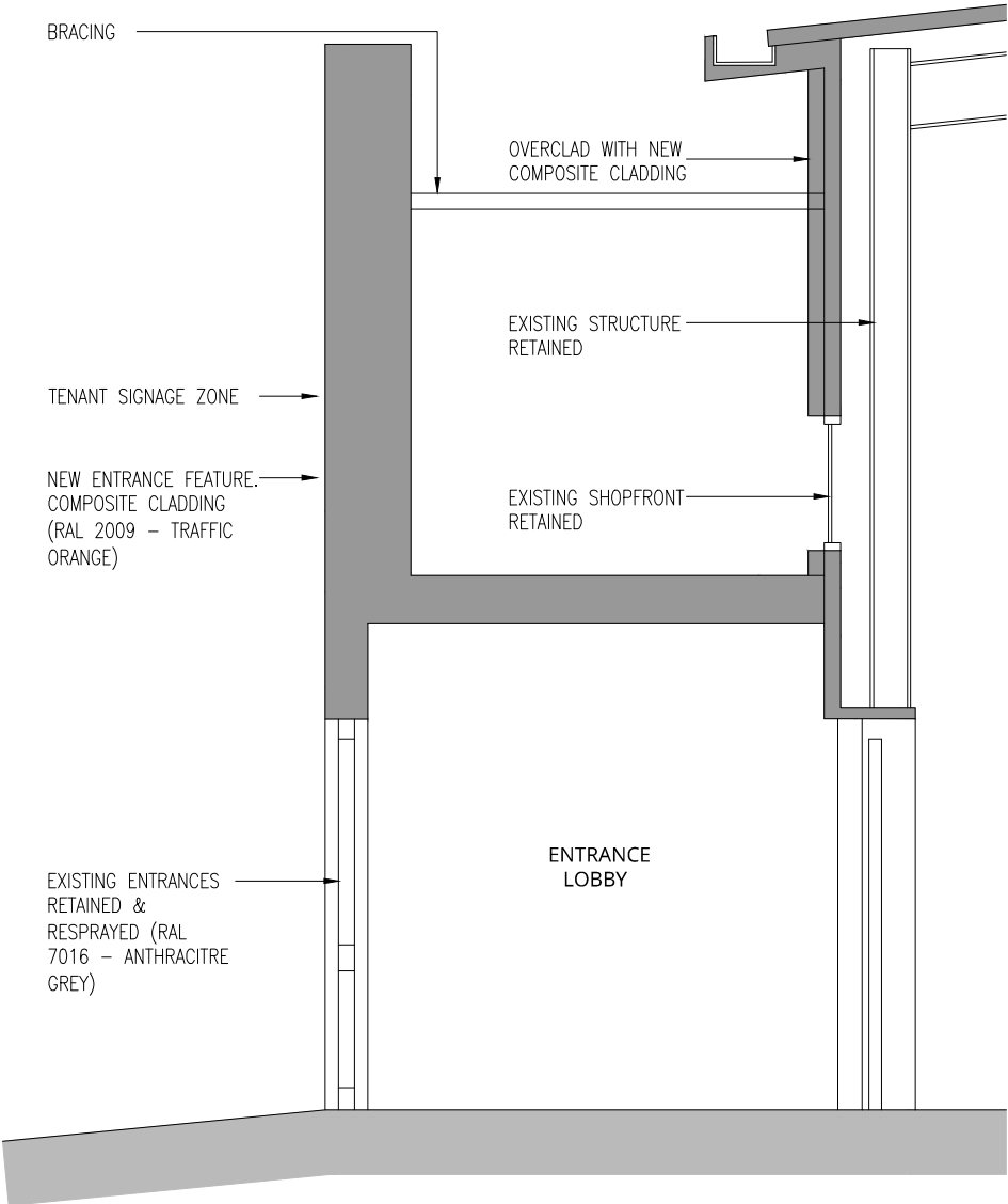
SECTION C-C (B&Q)
