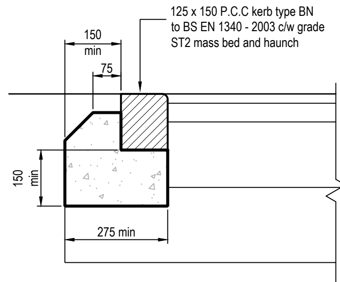
P.C.C. BN Drop Kerb Detail
