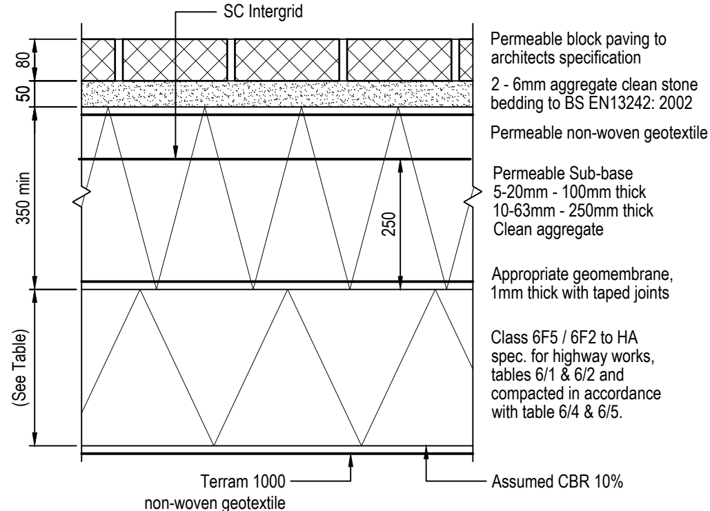
Type C - Permeable Block Paved Access Road Construction Detail Detail 2
