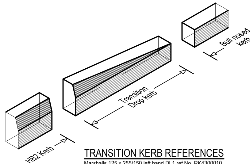
HB2 to BN Drop Kerb Typical
