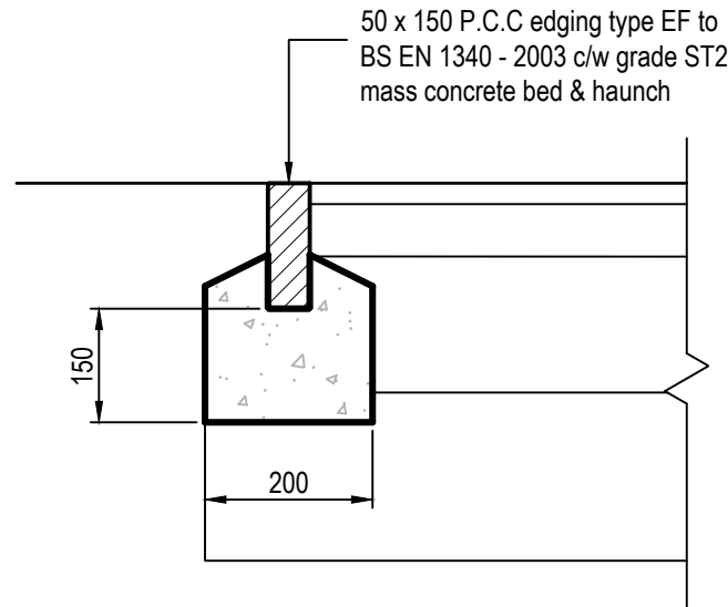
P.C.C. EF Edging Detail
