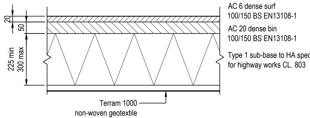
Macadam Footpath Construction Detail 5
