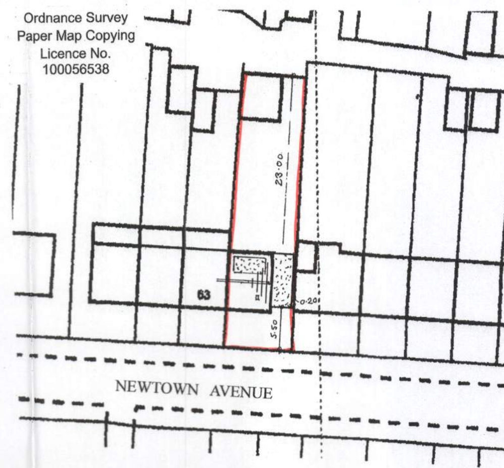
block plan
