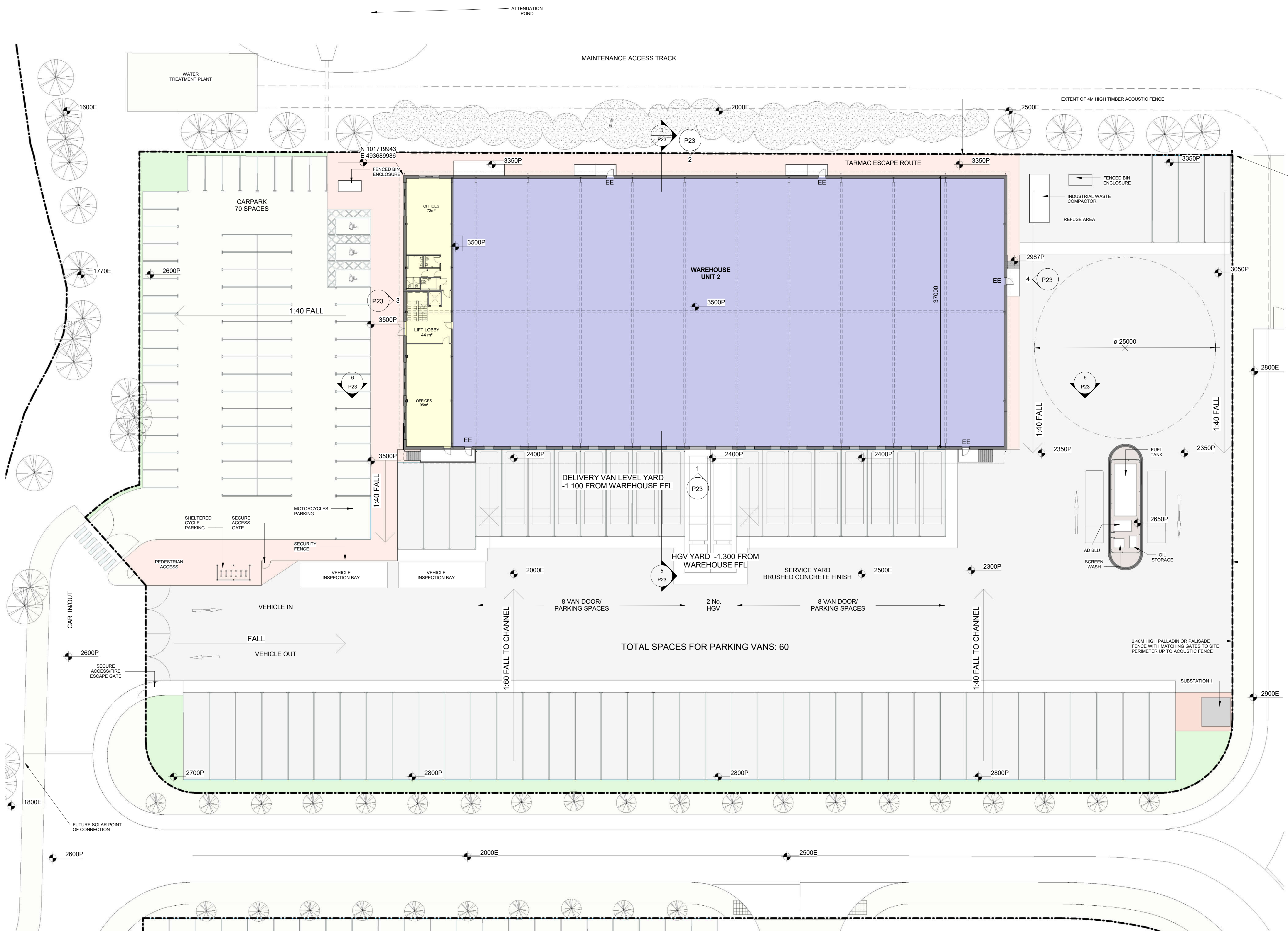
1 PROPOSED GROUND FLOOR PLAN 1 : 250
