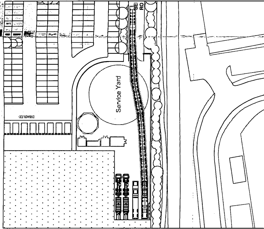
16.5m HGV exits site forward.
