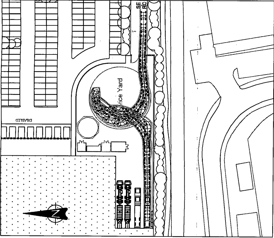
16.5m HGV accesses site forward and reverses into southern loading bay whilst all other bays are occupied.
