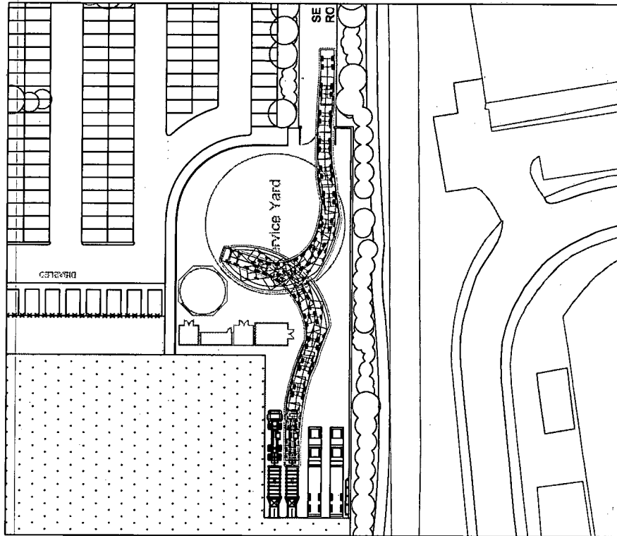
10.2m Waste Lorry accesses the site forward and performs a reverse manoeuvre into the southern compactor bay whilst all other bays are occupied.
