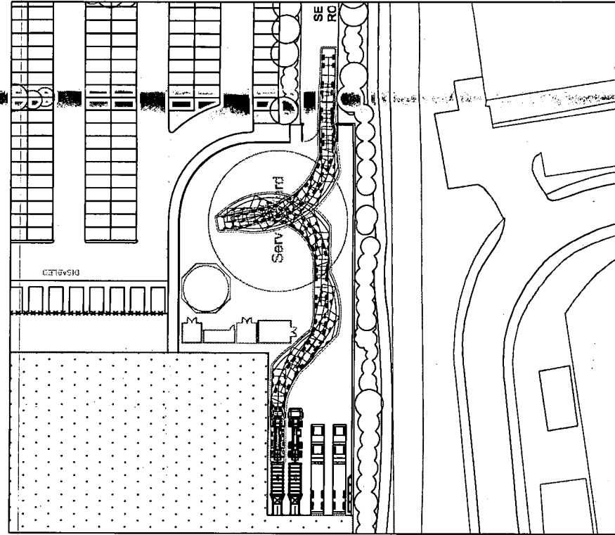
10.2m Waste Lorry accesses the site forward and performs a reverse manoeuvre into the northern compactor bay whilst all other bays are occupied.
