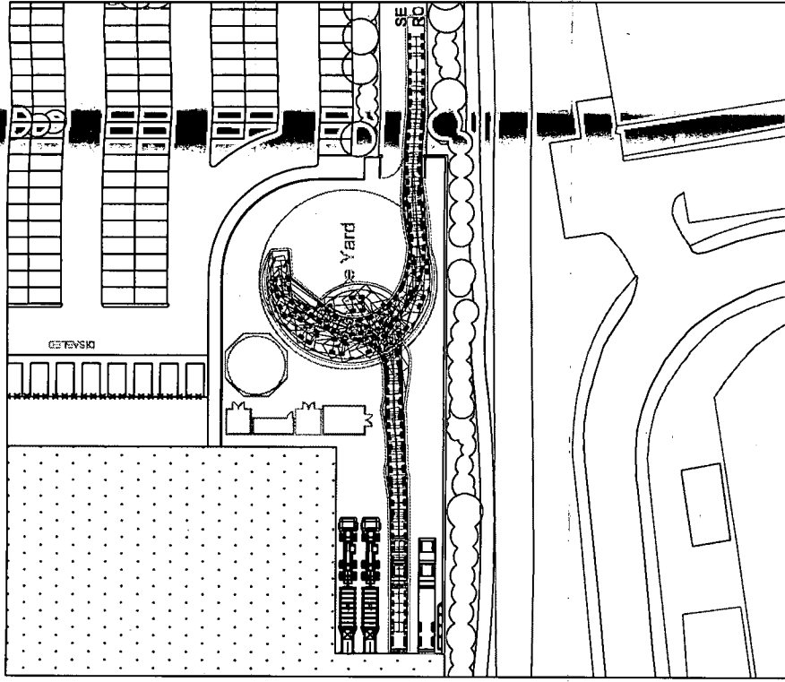
16.5m HGV accesses site forward and reverses into northern loading bay whilst all other bays are occupied.
