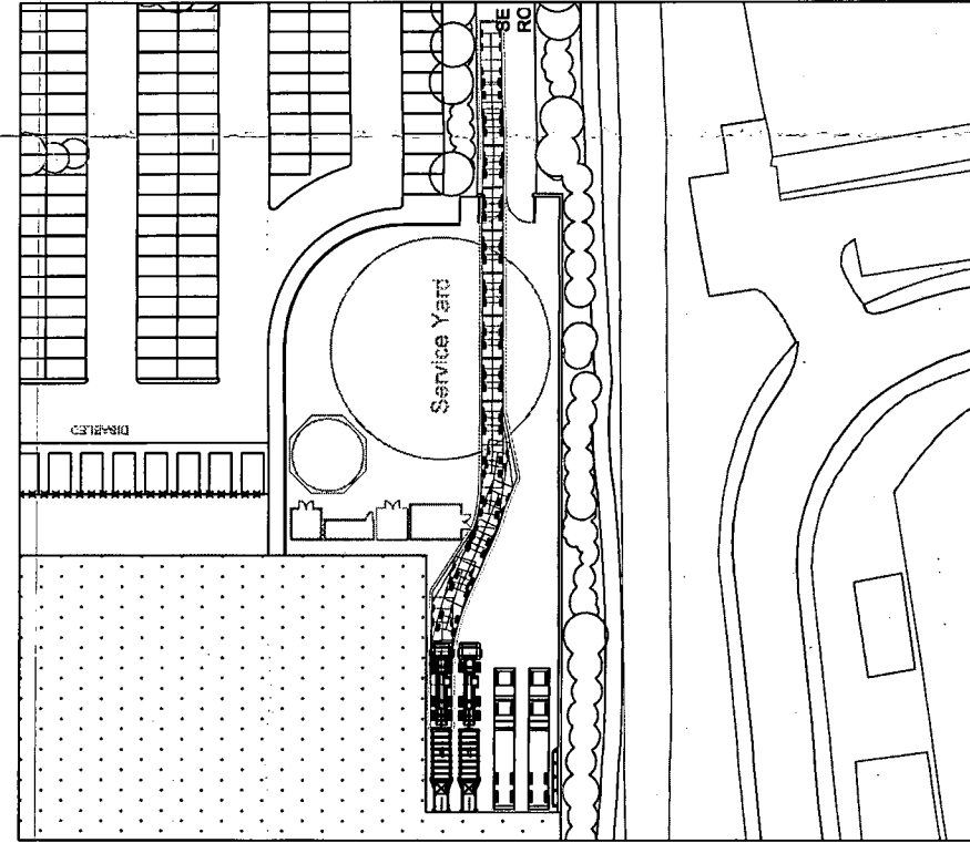
10.2m Waste Lorry exits site forward.
