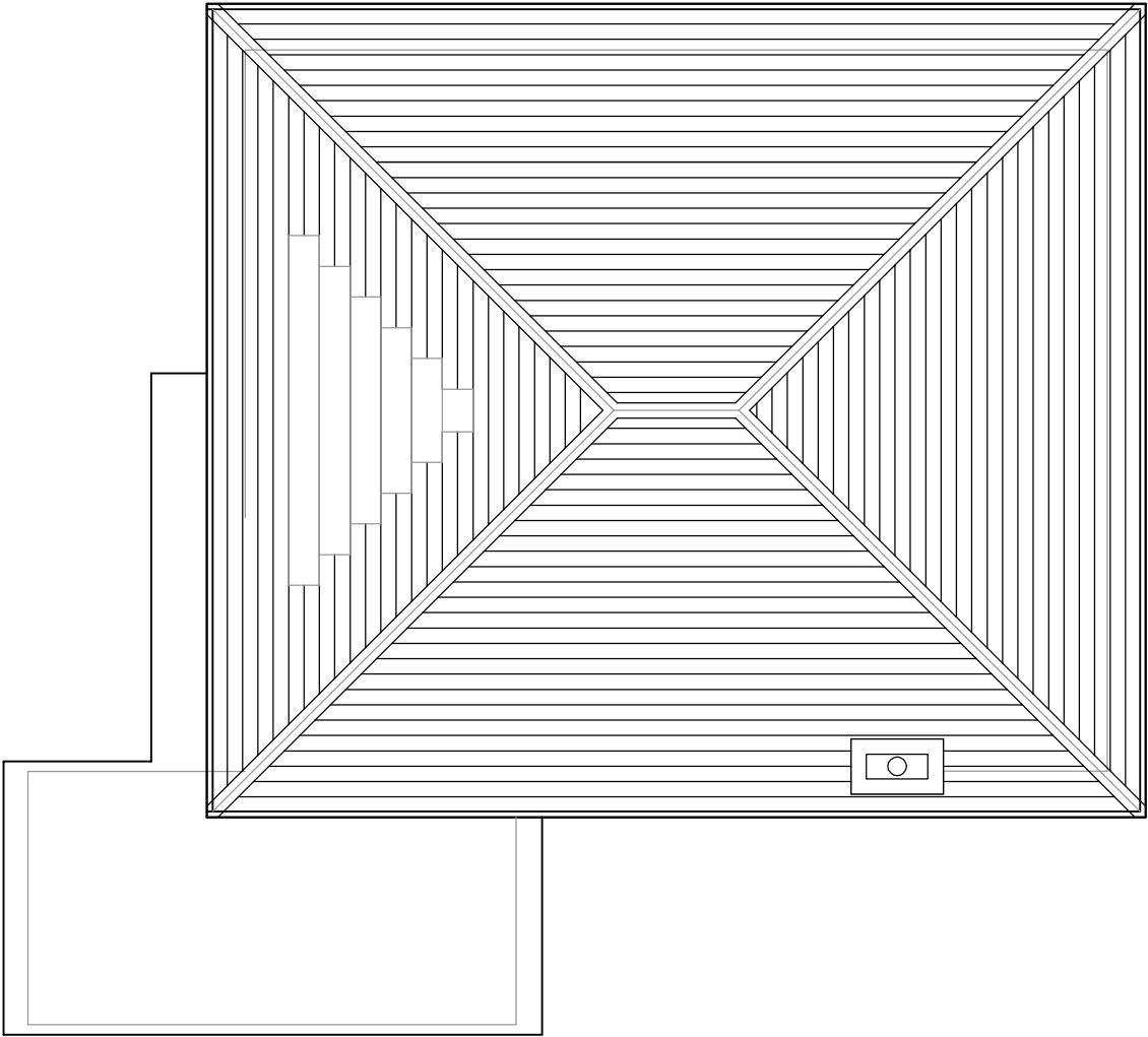
Roof Plan
