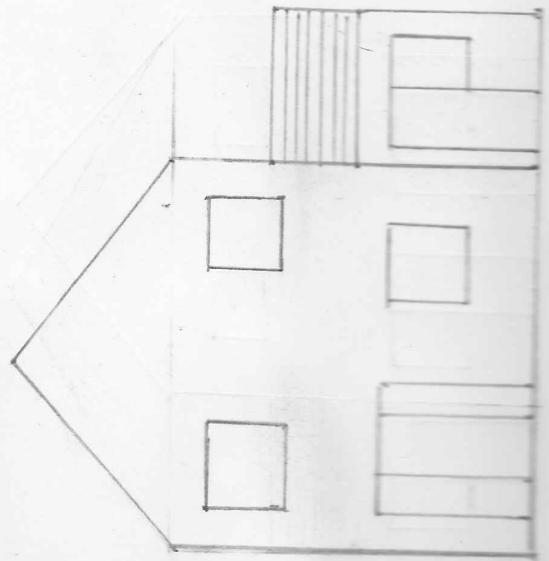
EXISTING EAST ELEVATION
