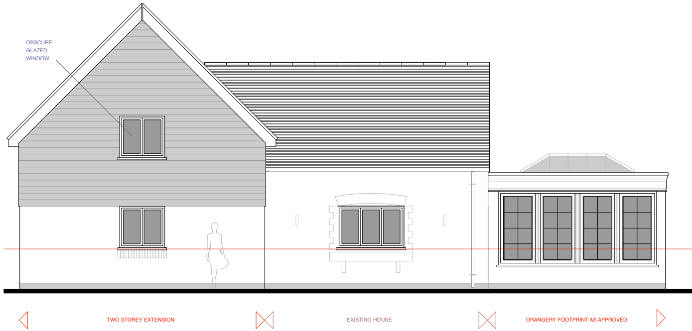
Proposed Side Elevation at 1:100 scale SOUTH EAST
