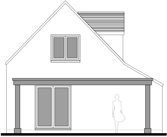
Existing Side Elevation at 1:100 scale
