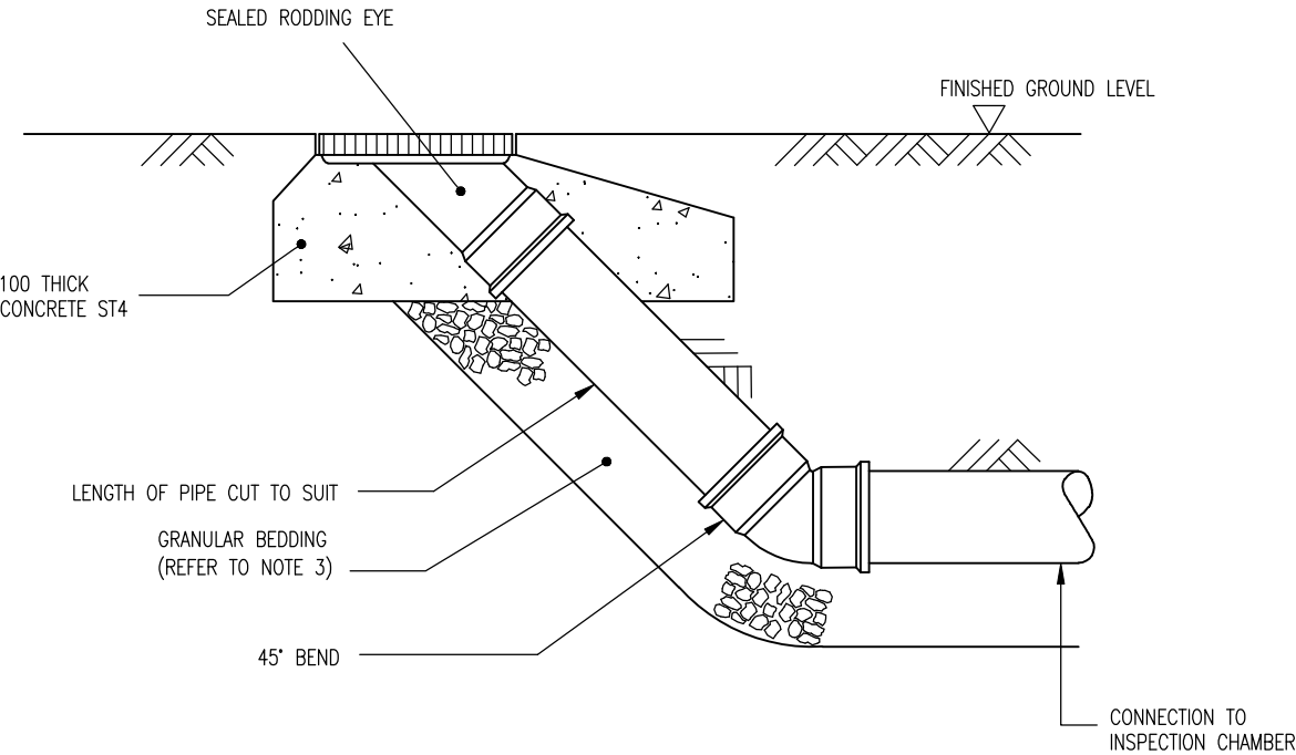
SEALED RODDING EYE
