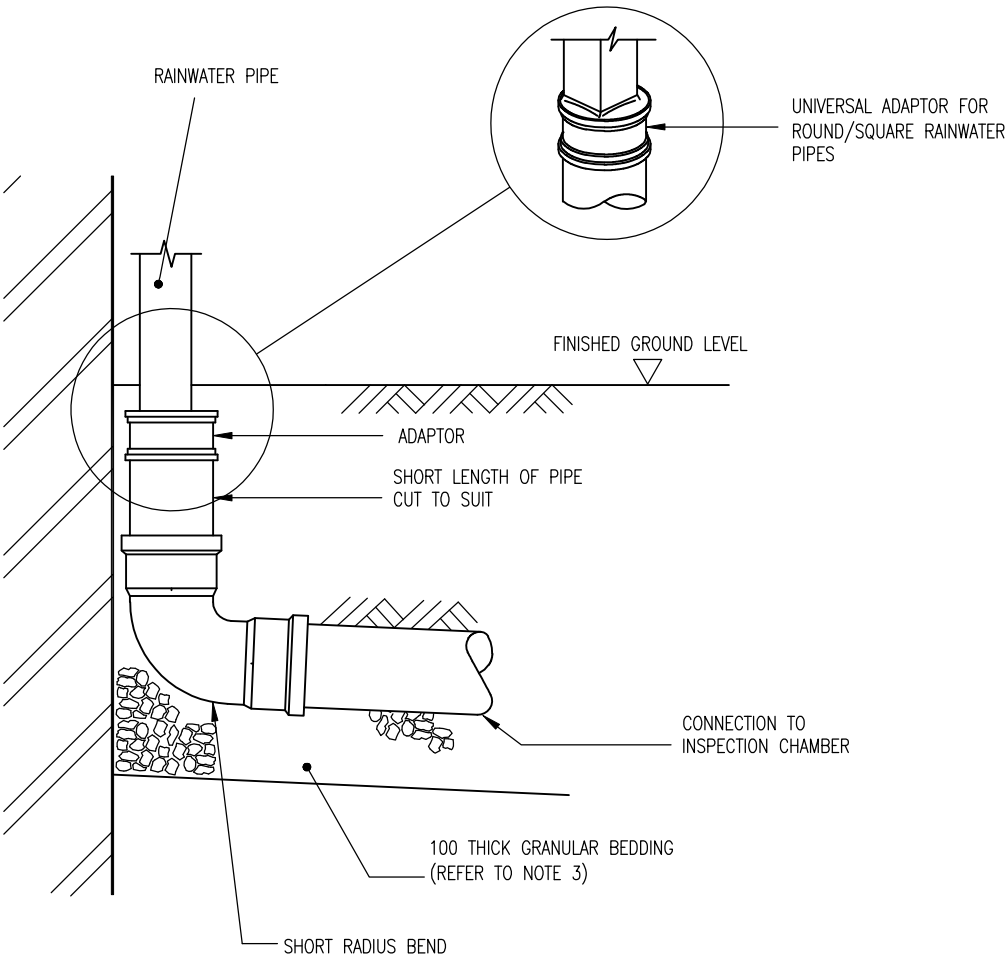
RAINWATER PIPE CONNECTED TO INSPECTION CHAMBER
