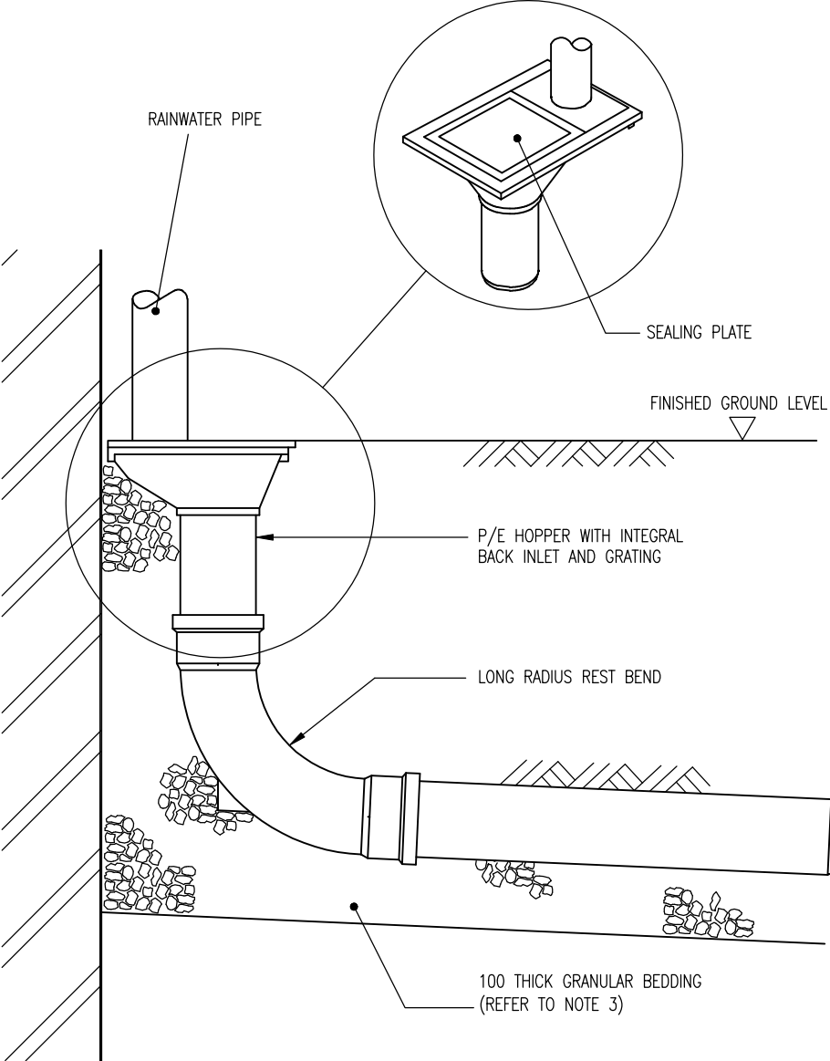
RAINWATER PIPE CONNECTED TO COLLECTOR DRAIN VIA A JUNCTION
