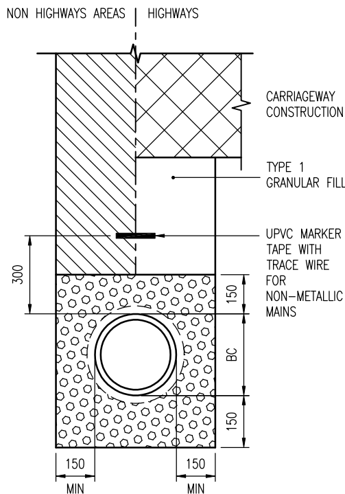
RISING MAIN
