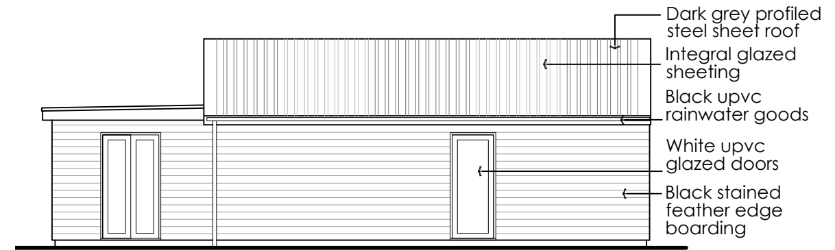
North East elevation 1:100 @ A3
