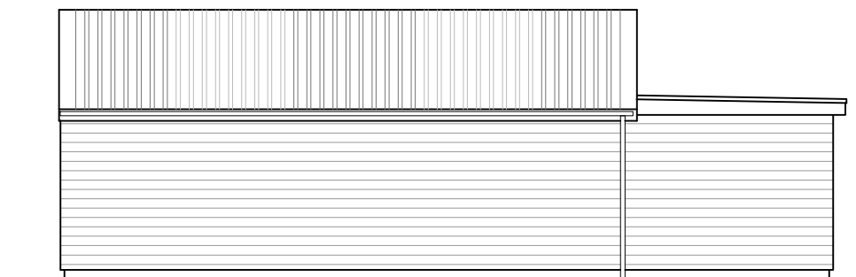
South West elevation 1:100 @ A3
