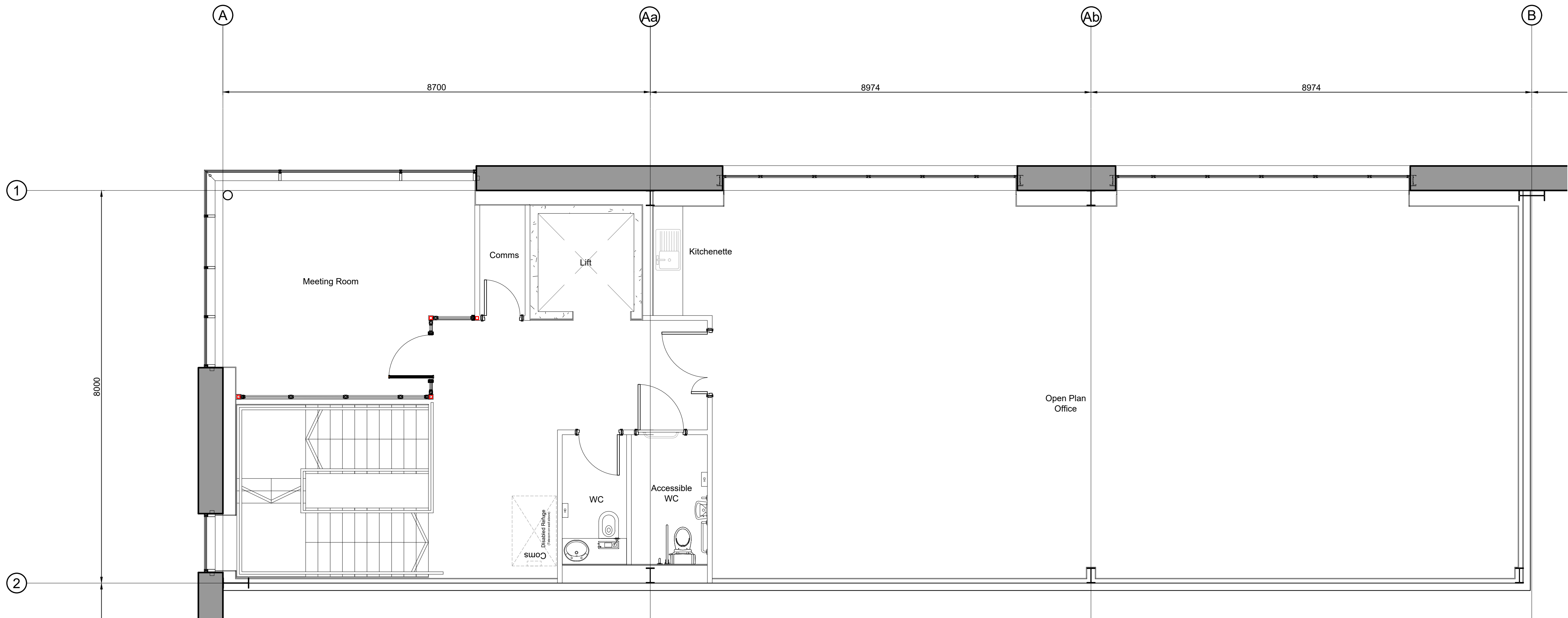
Unit 1 First Floor Office Layout Scale 1:50
