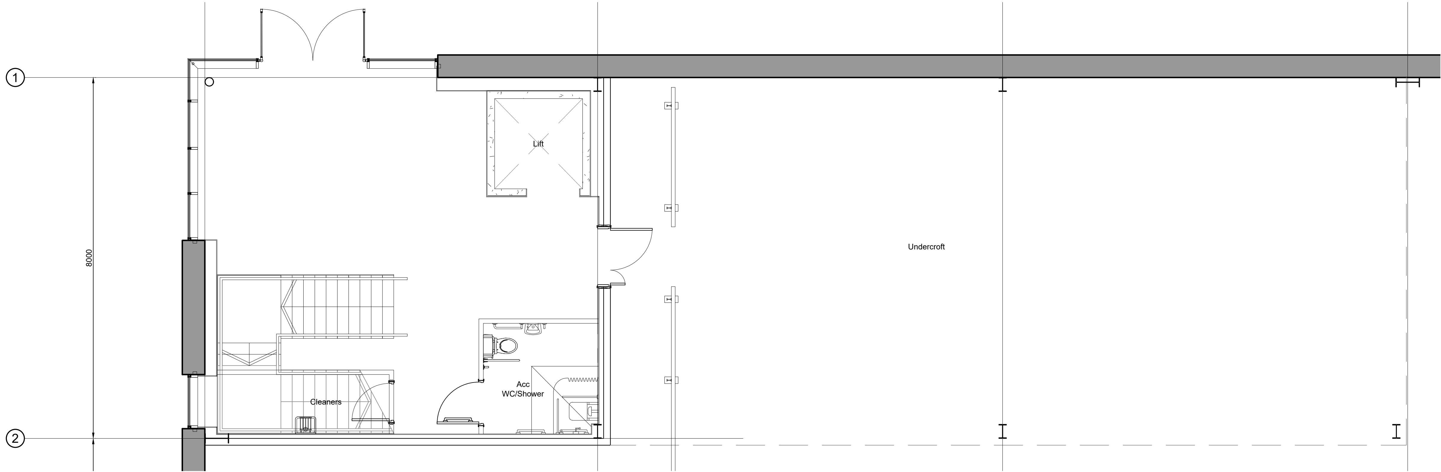
Unit 1 Ground Floor Office Layout Scale 1:50
