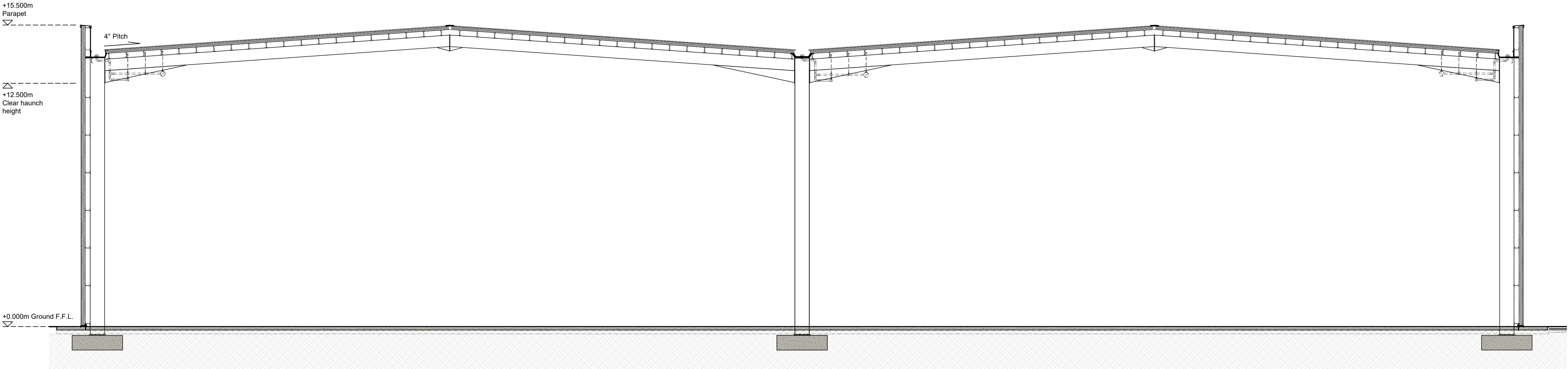
Warehouse Section Scale 1:100
