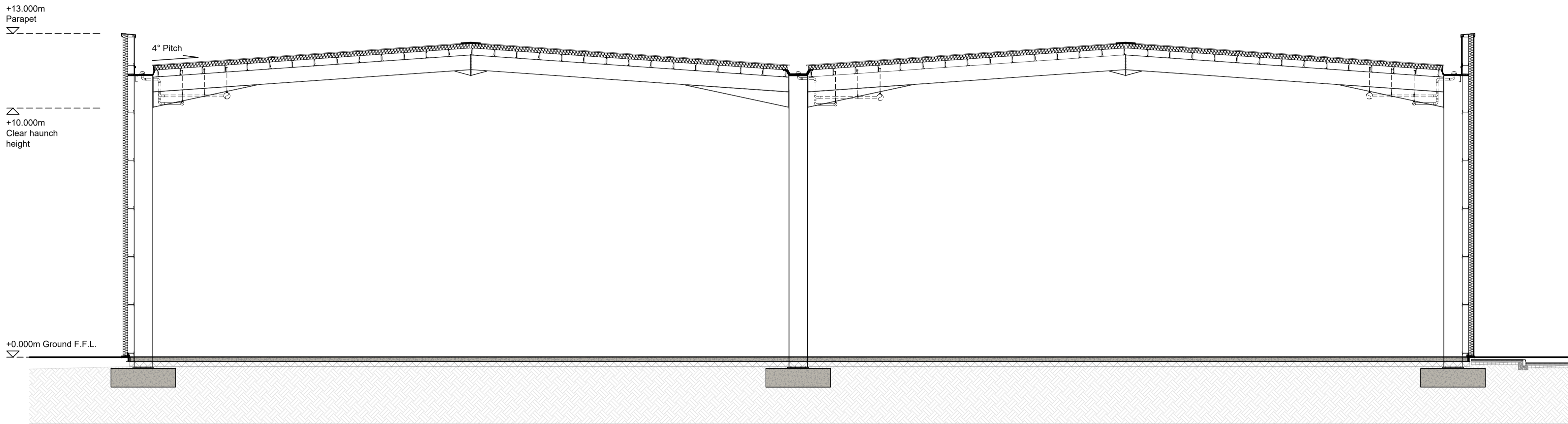
Warehouse Section Scale 1:100
