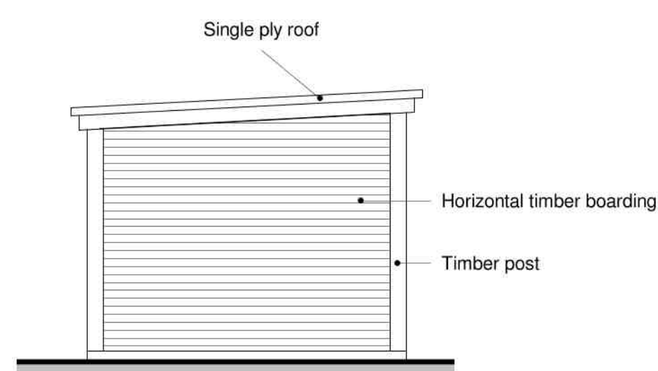
8 Elevation Garden Room South 1 : 50
