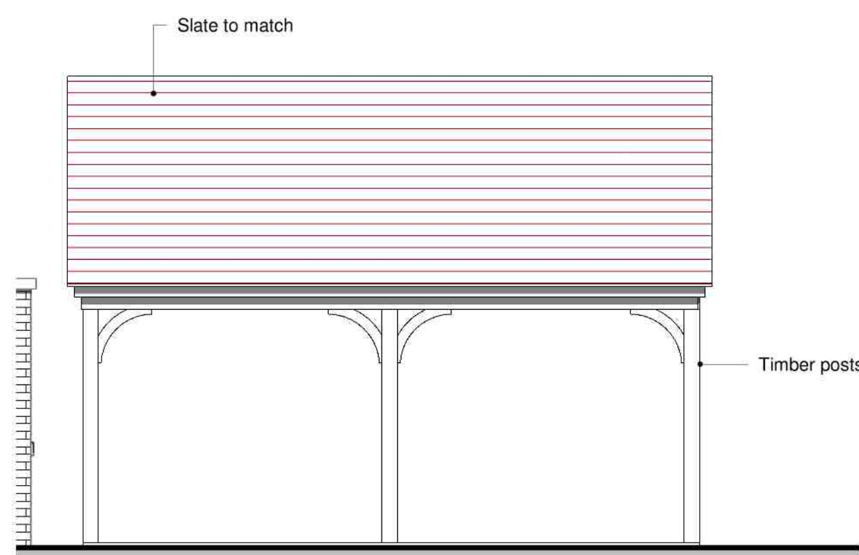
2 Elevation Carport Rear South 1 : 50
