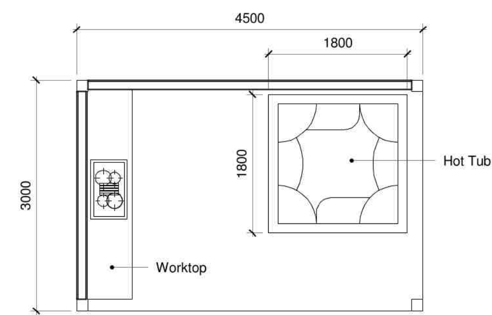
12 FFL Ground Proposed Garden Room 1 : 50
