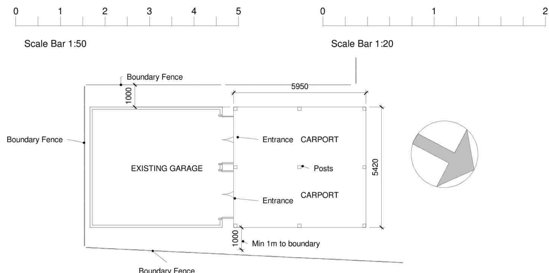
11 FFL Ground Proposed Carport 1 : 100
