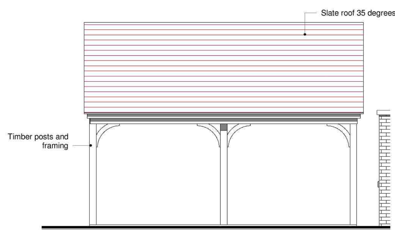
4 Elevation Carport Side West 1 : 50
