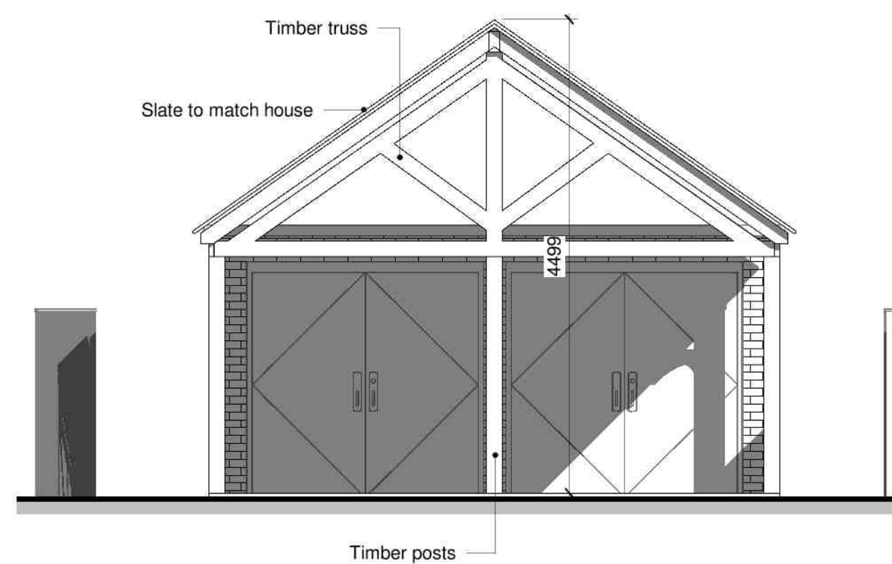
1 Elevation Carport Front North 1 : 50
