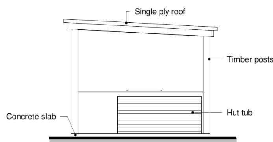
7 Elevation Garden Room North 1 : 50
