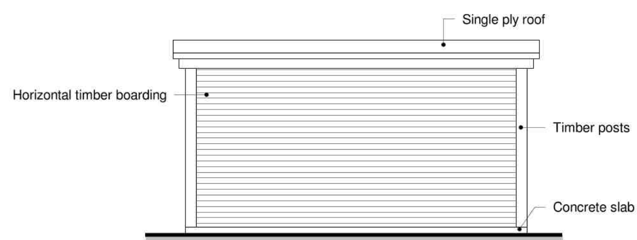
10 Elevation Garden Room West 1 : 50
