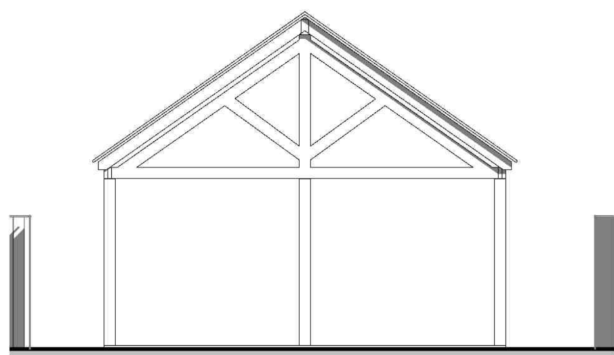
2 Elevation Carport Rear South 1 : 50
