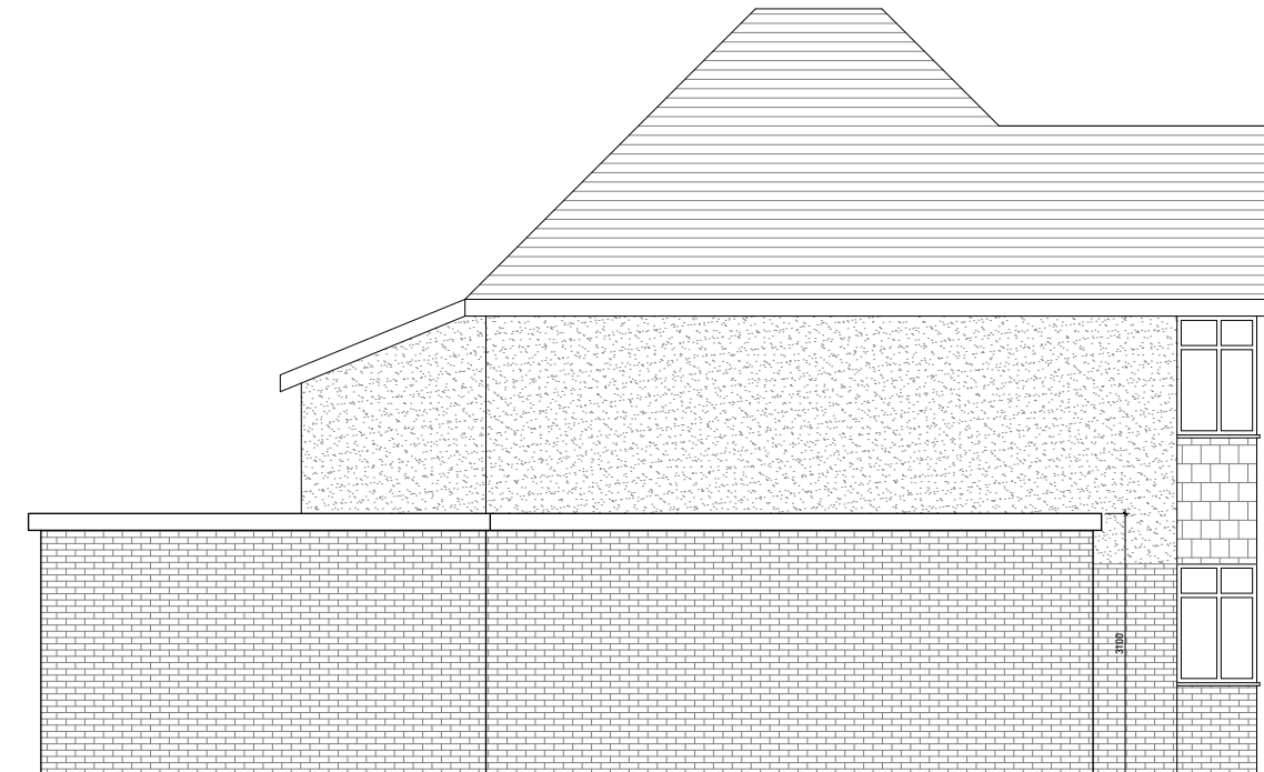
PROPOSED SIDE ELEVATION 1:50
