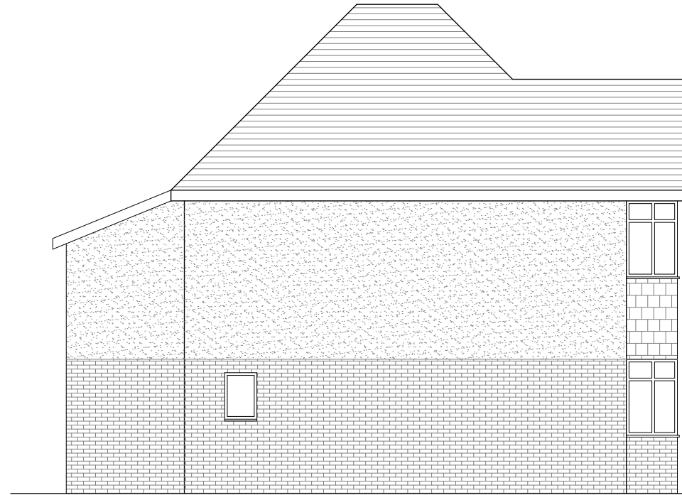
EXISTING SIDE ELEVATION 1:50
