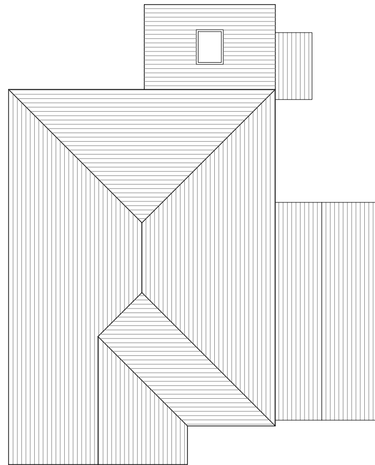
EXISTING ROOF PLAN 1:50
