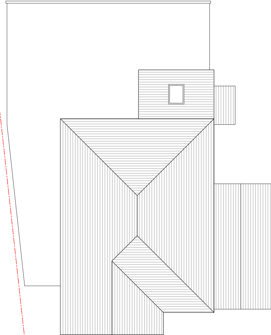
PROPOSED ROOF PLAN 1:50
