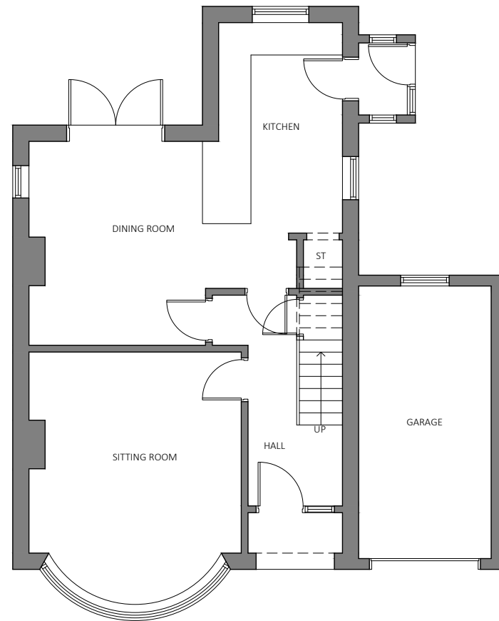
EXISTING GROUND FLOOR PLAN 1:50
