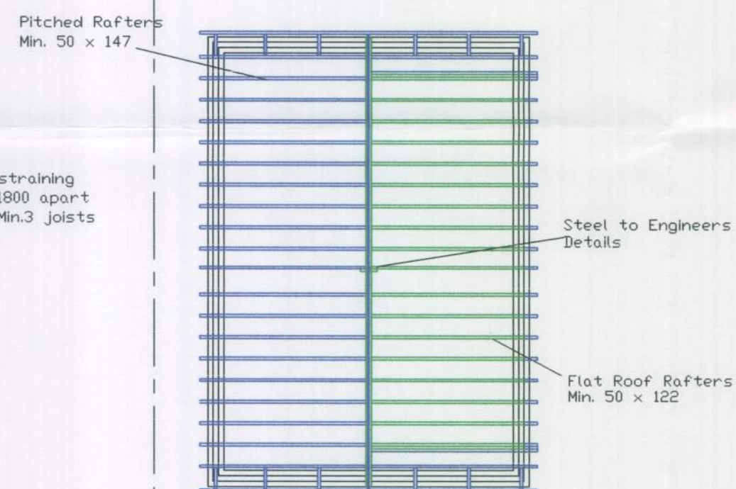
Proposed Rafters and steel Plan
