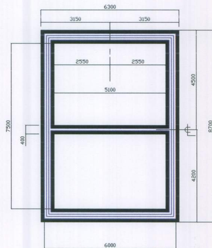
Plan of Concrete Foundations showing cavity wall line
