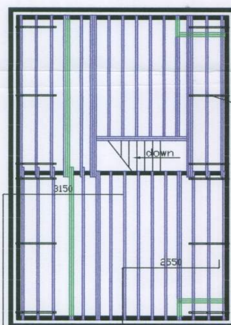
Plan of First Floor Joists
