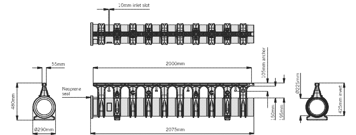
ACO Qmax® 225 with ACO Q-Guard galvanised steel edge rail
