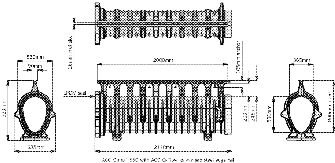
ACO Qmax® 550 with ACO Q-Flow galvanised steel edge rail
