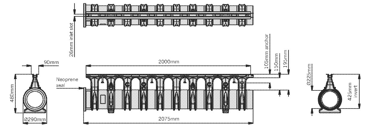
ACO Qmax® 225 with ACO Q-Flow galvanised steel edge rail
