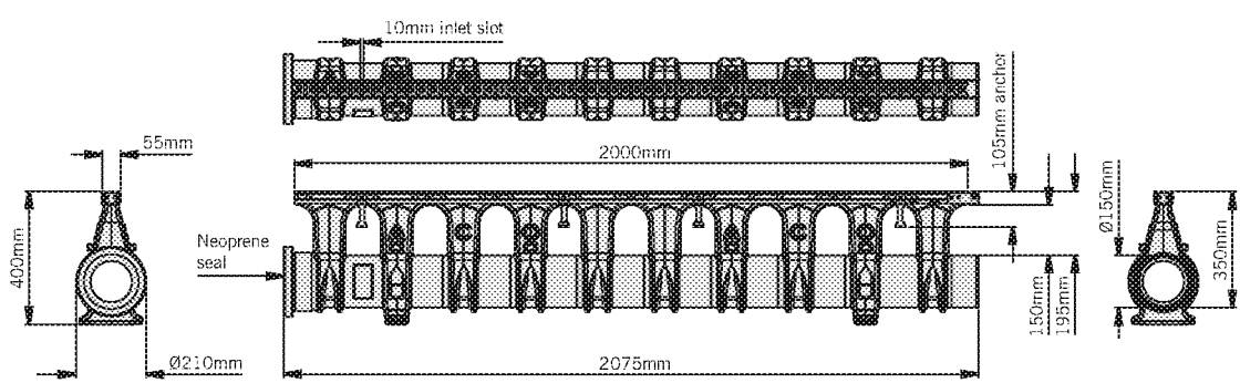
ACO Qmax® 150 with ACO Q-Guard galvanised steel edge rail
