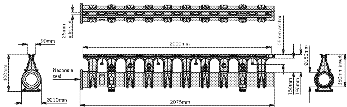
ACO Qmax® 150 with ACO Q-Flow galvanised steel edge rail
